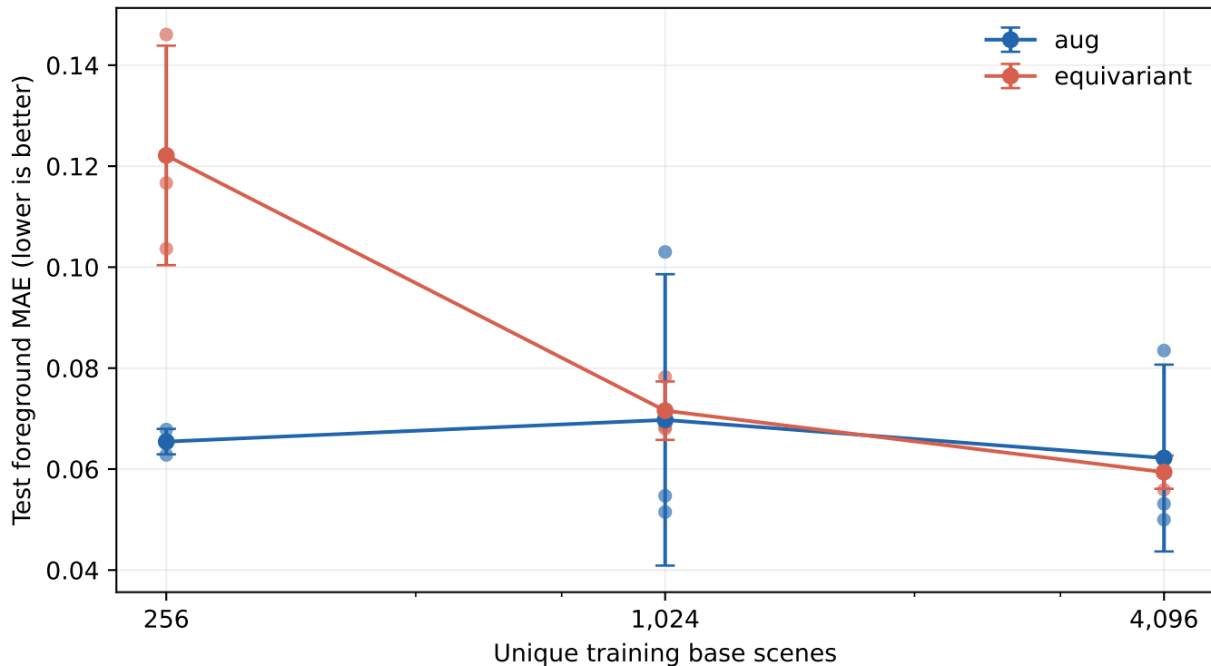
Same 3,000 optimizer steps; 3 initialization seeds
