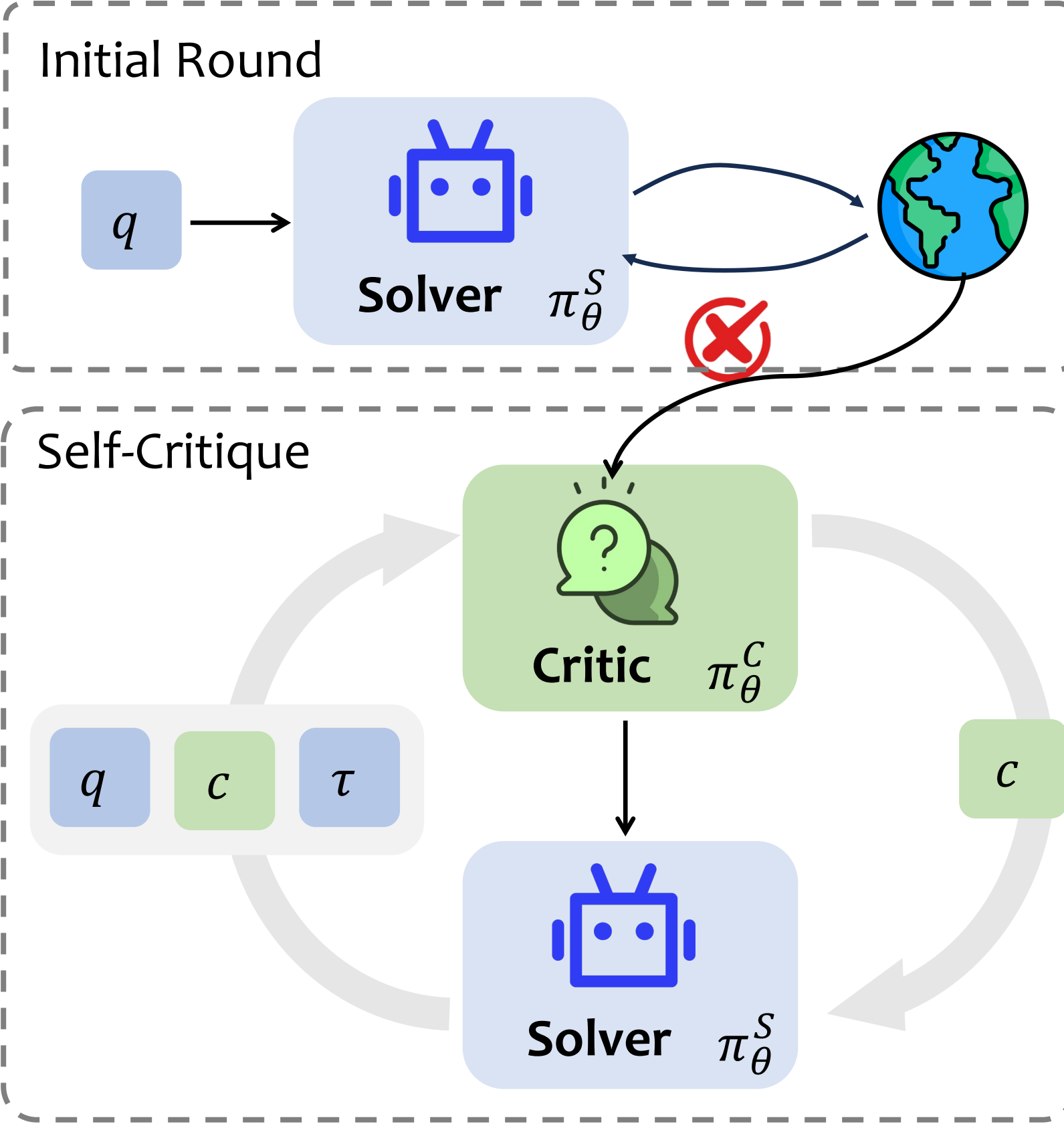
(a) Rollout w/ Critique
