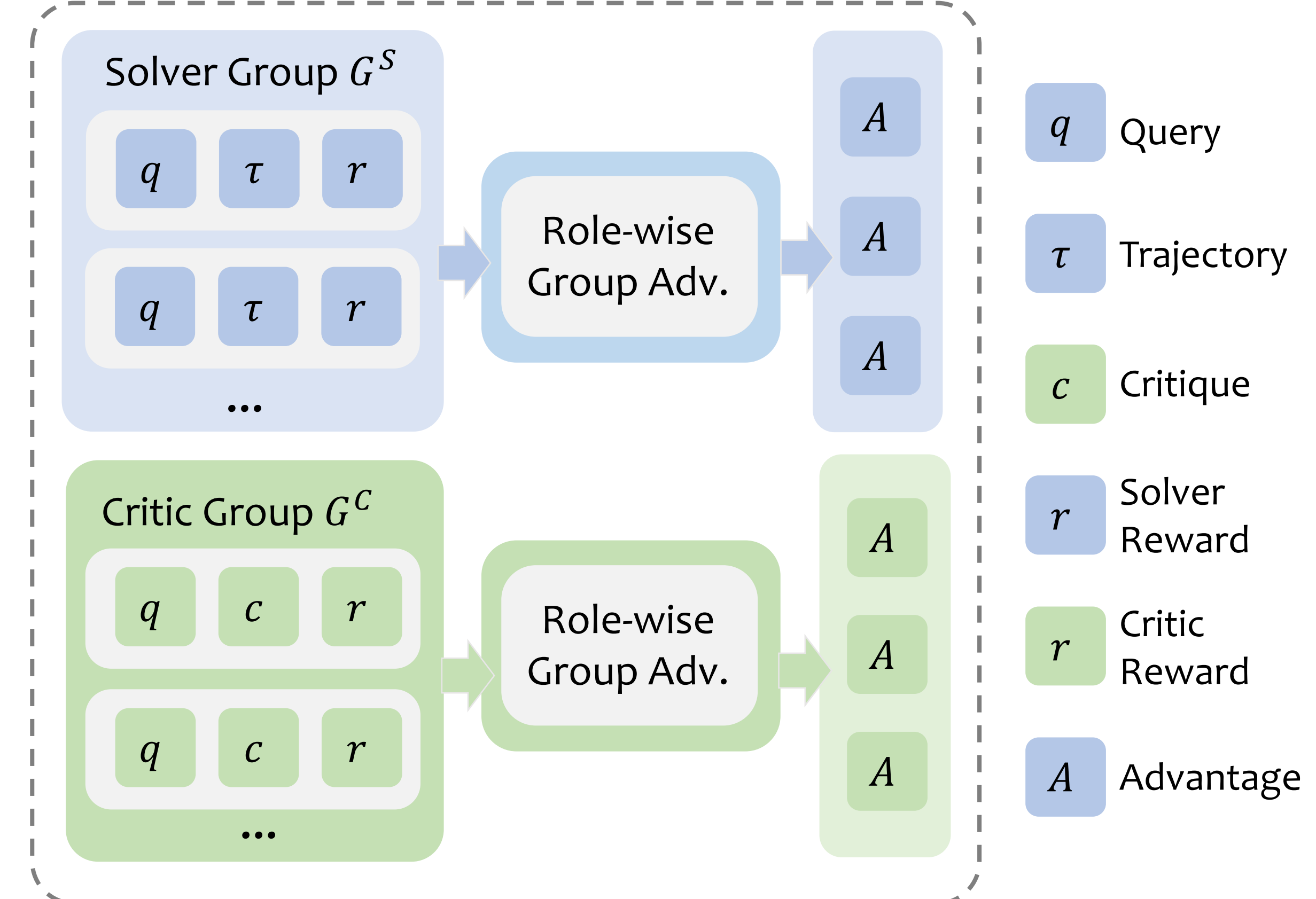
(c) Policy Optimization
