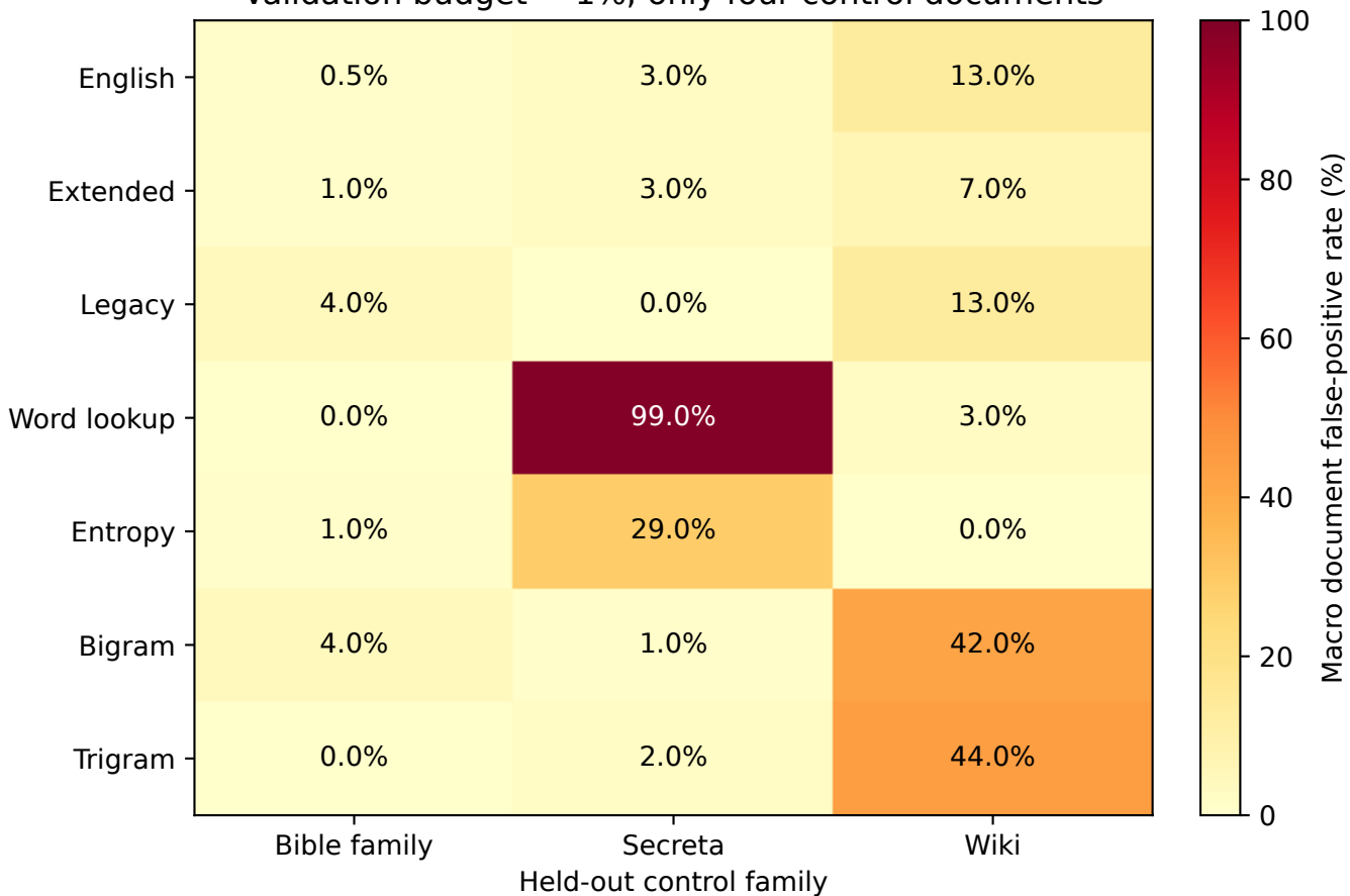
Calibration transfer: test false-positive rate Validation budget = 1%; only four control documents
