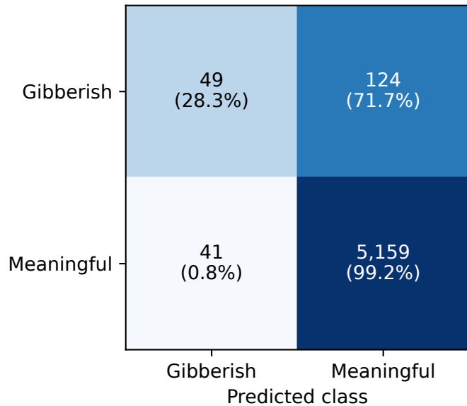
English Accuracy 96.93%
