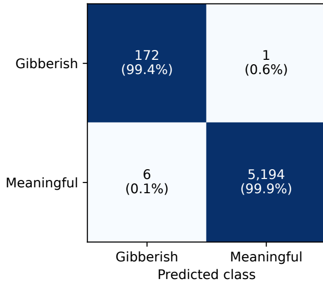
HF noise/salad Accuracy 99.87%
