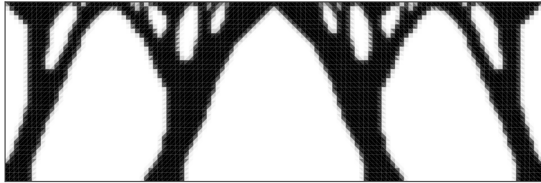
(b) LFEM ( p = 1 , \nu_0 = 0.4999 , C = 76.43 )
