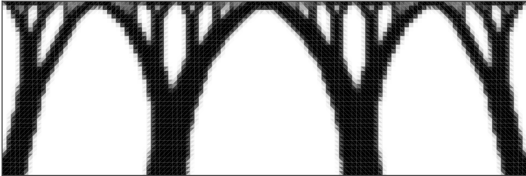
(c) LFEM ( p = 2 , \nu_0 = 0.30 , C = 122.73 )
