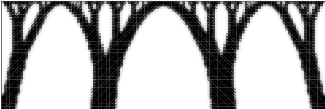
(a) LFEM ( p = 1 , \nu_0 = 0.30 , C = 119.33 )
