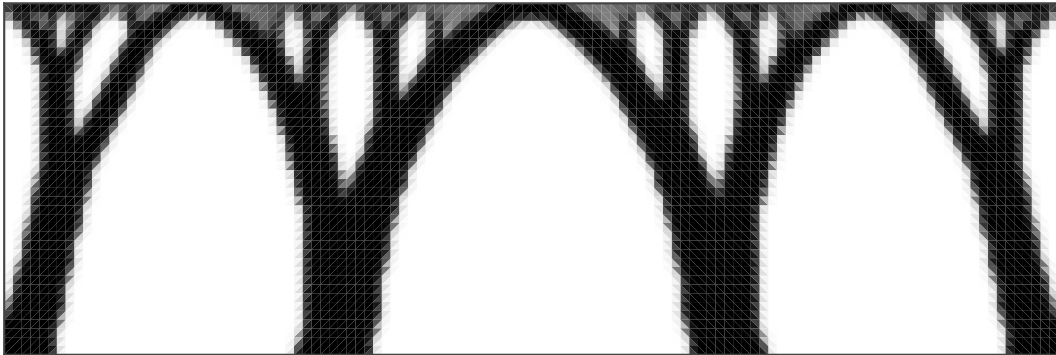
(e) HZMFEM ( k = 2 , \nu_0 = 0.30 , C = 127.68 )
