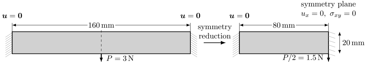
(a) full domain \Omega
