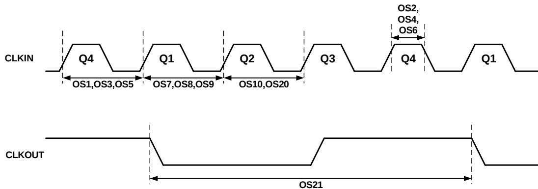
Figure 43-4. Clock Timing
