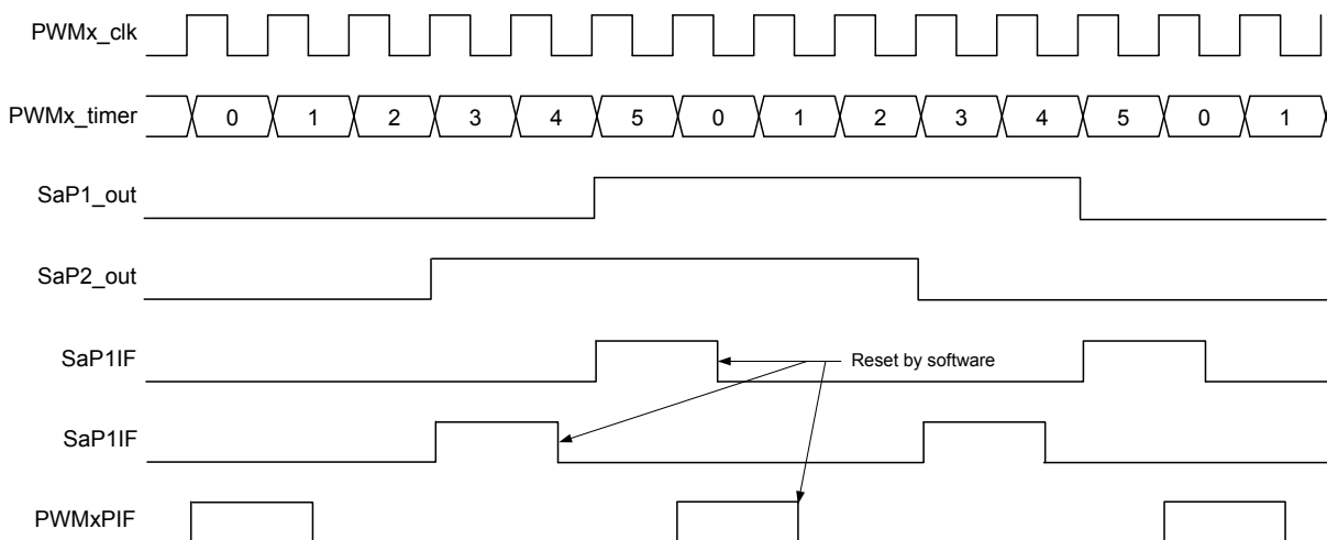
Figure 29-12. Toggled Compare Timing Diagram
