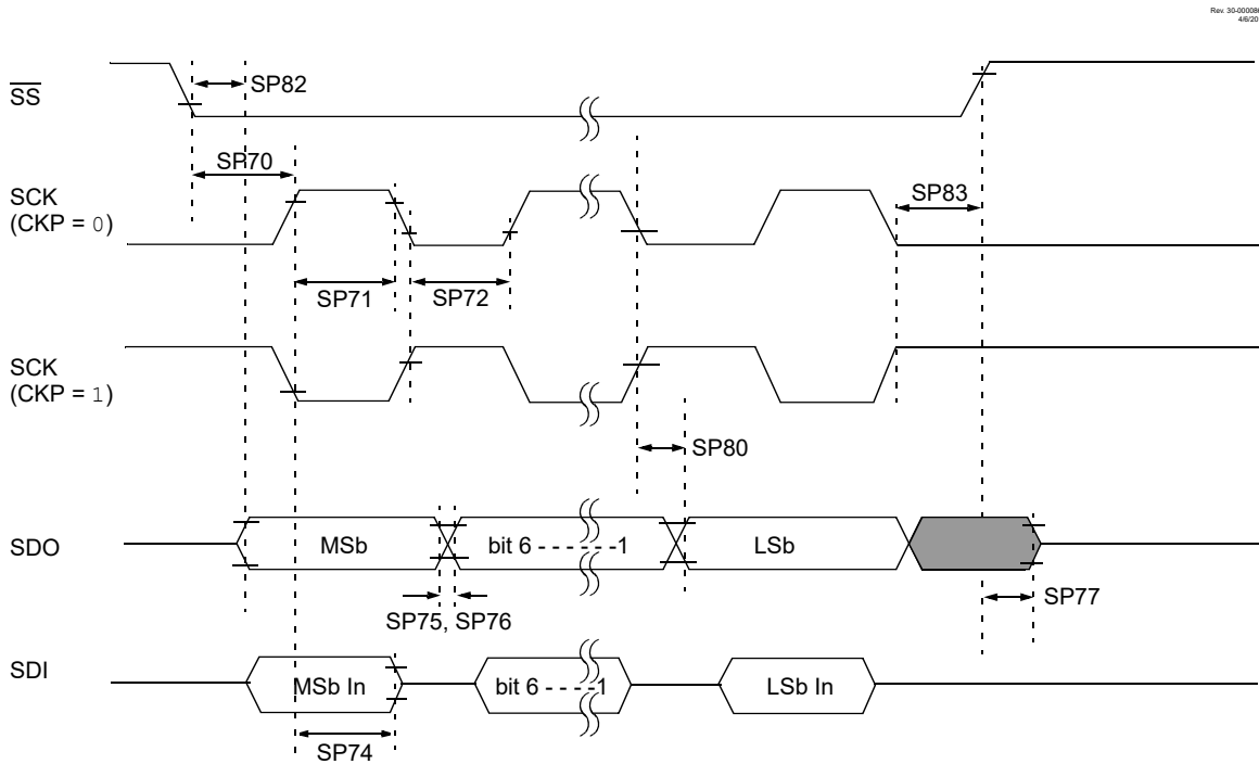
Figure 42-18. SPI Client Mode Timing (CKE = 1)
