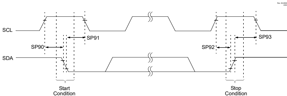
Figure 42-19. I 2 C Bus Start/Stop Bits Timing
