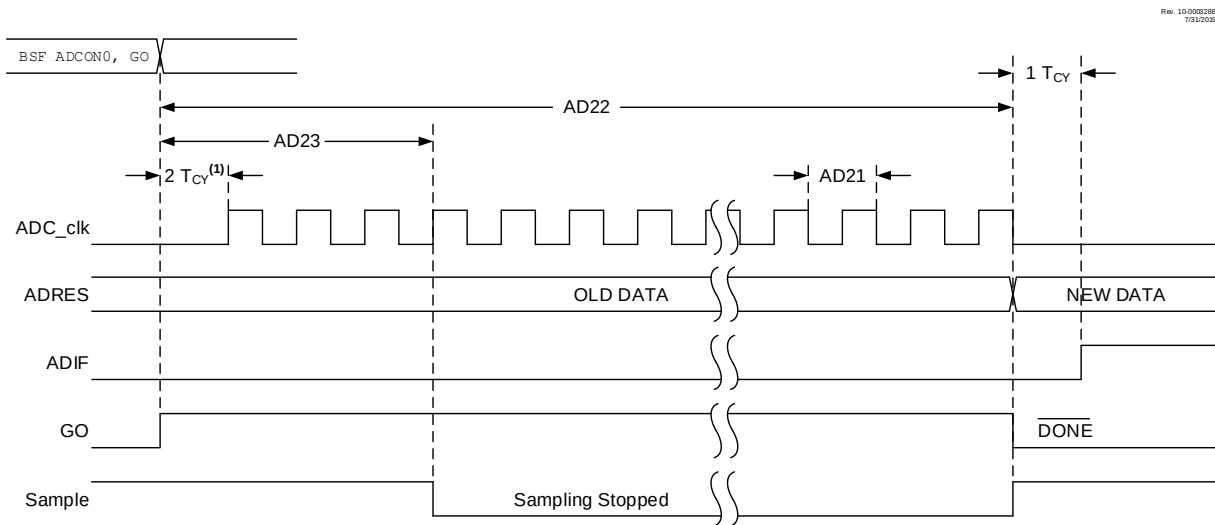
Figure 42-10. ADC Conversion Timing (ADC Clock from F_{RC} )
