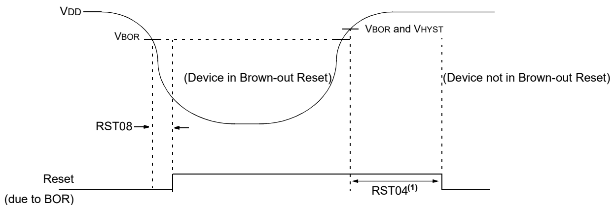
Figure 42-8. Brown-out Reset Timing and Characteristics
