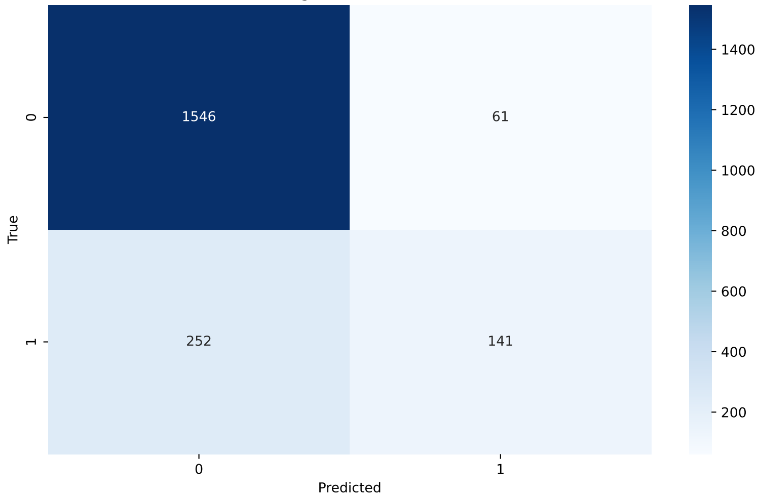
K-Nearest Neighbors - Confusion Matrix
