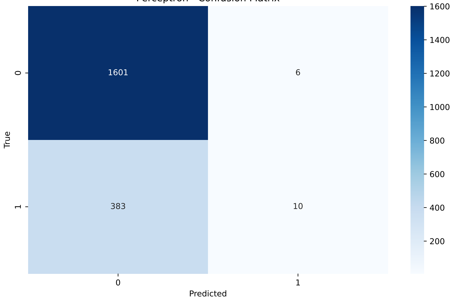
Perceptron - Confusion Matrix
