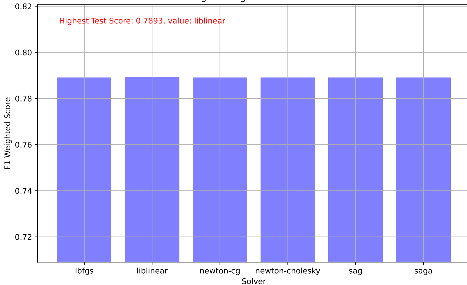
Logistic Regression - Solver
