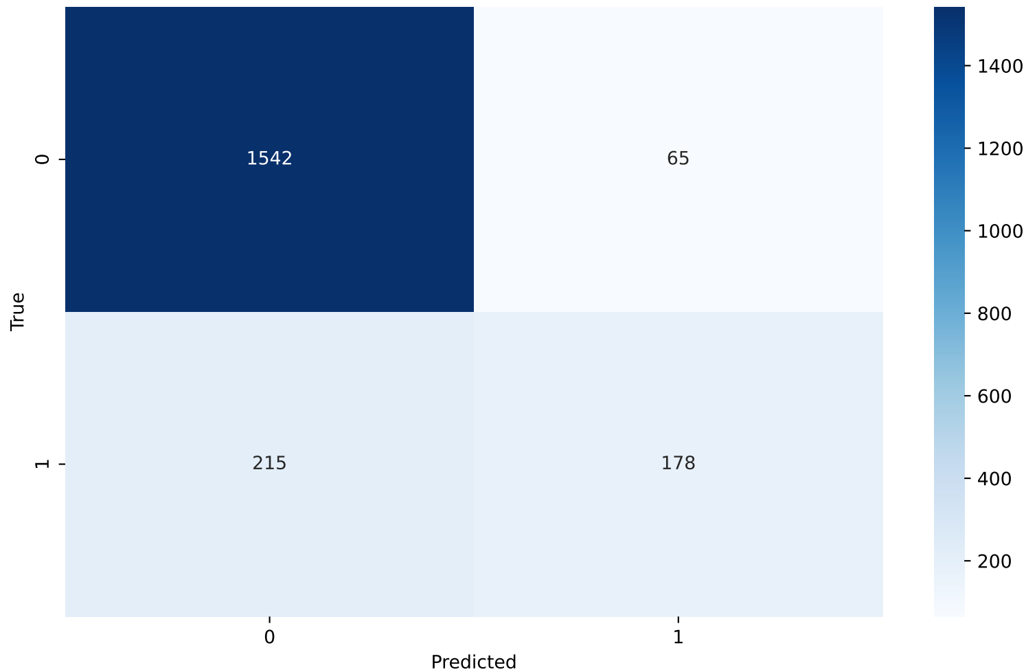
Decision Tree - Confusion Matrix
