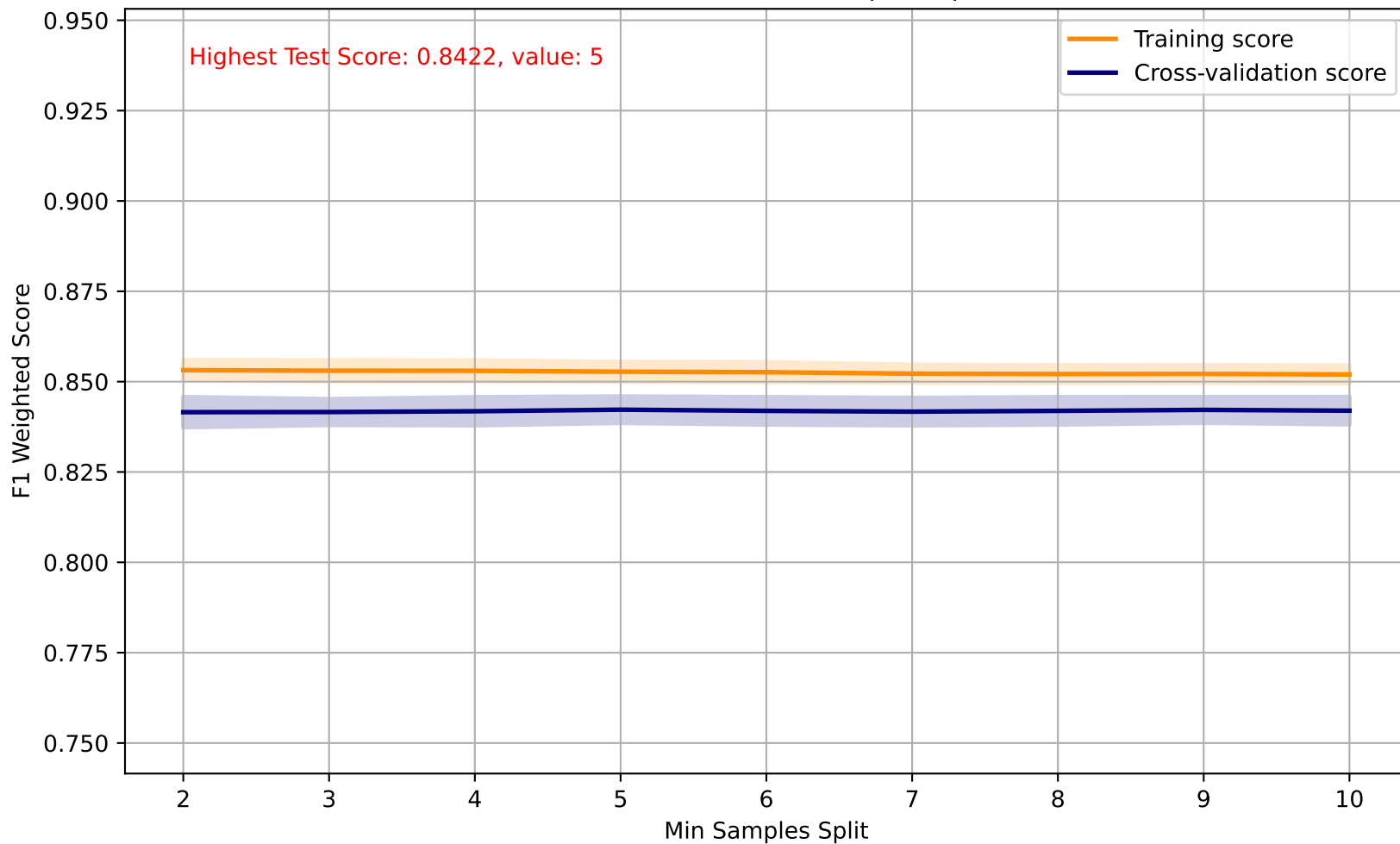
Decision Tree - Min Samples Split
