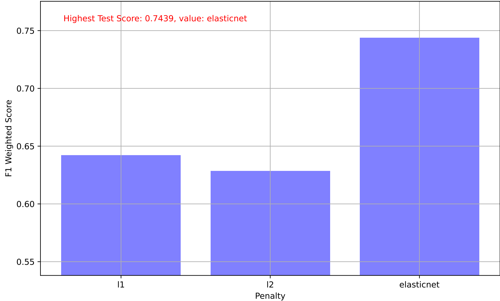
Perceptron - Penalty
