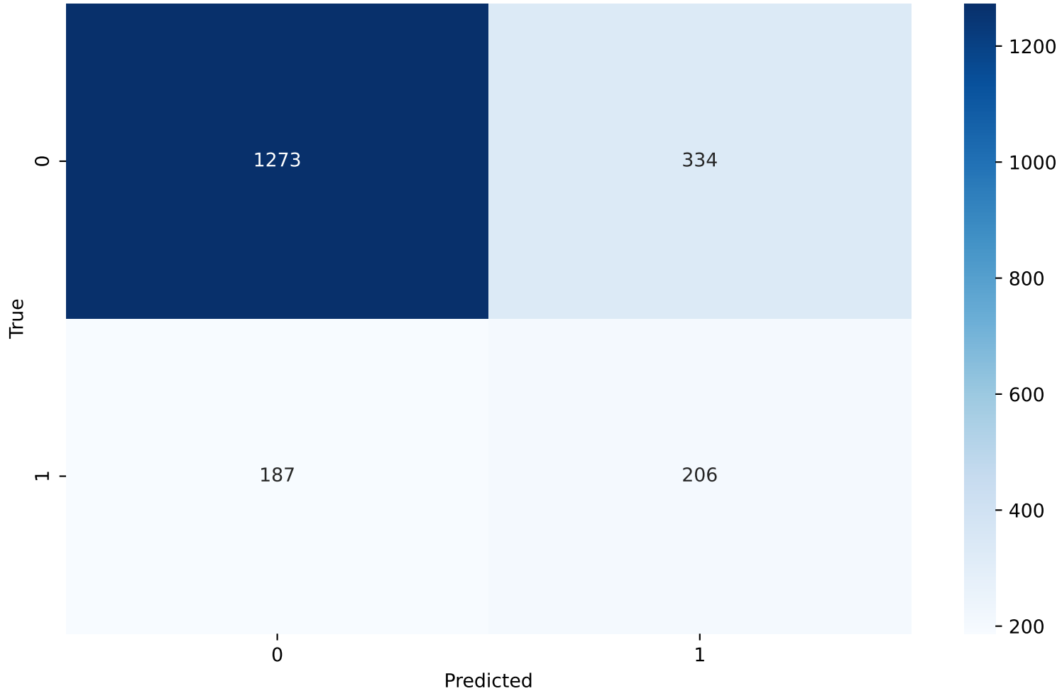
Perceptron - Confusion Matrix
