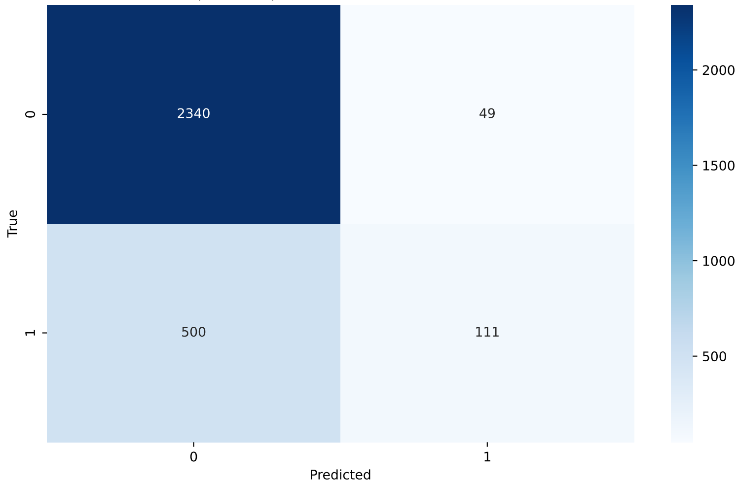
Perceptron - Alpha - Confusion Matrix(0.00011)
