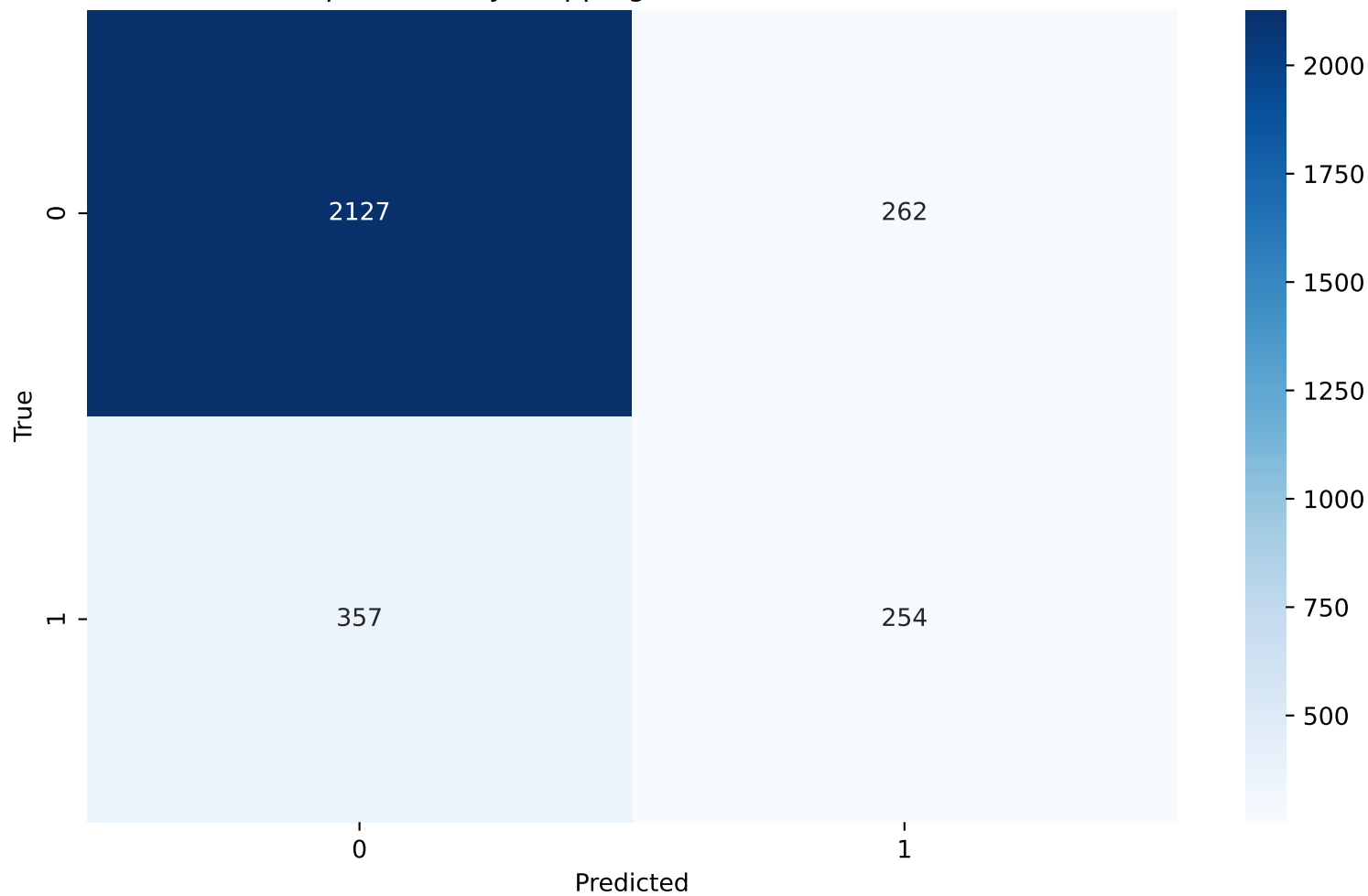
Perceptron - Early Stopping - Confusion Matrix(False)
