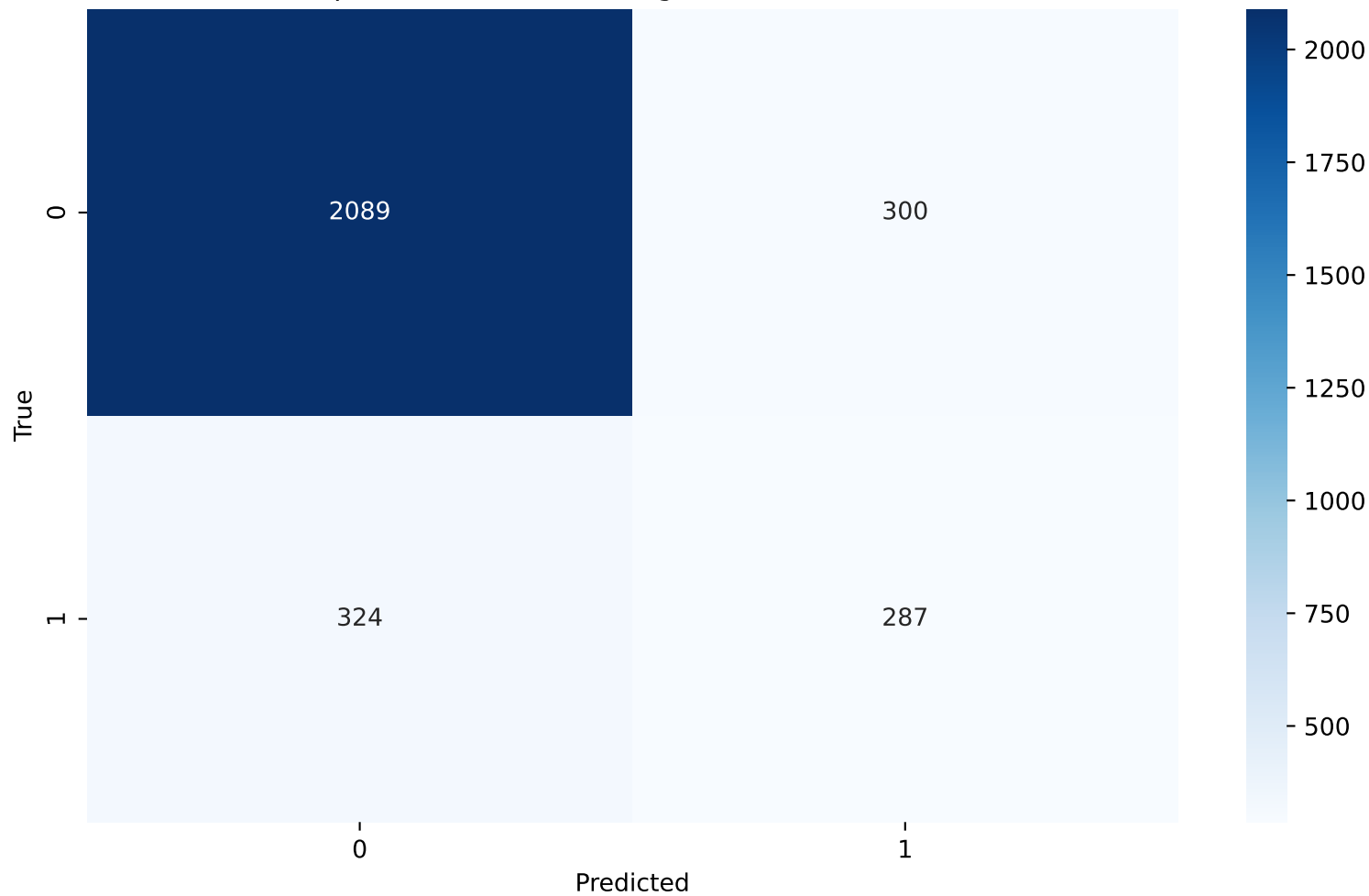
Perceptron - N Iter No Change - Confusion Matrix(5)
