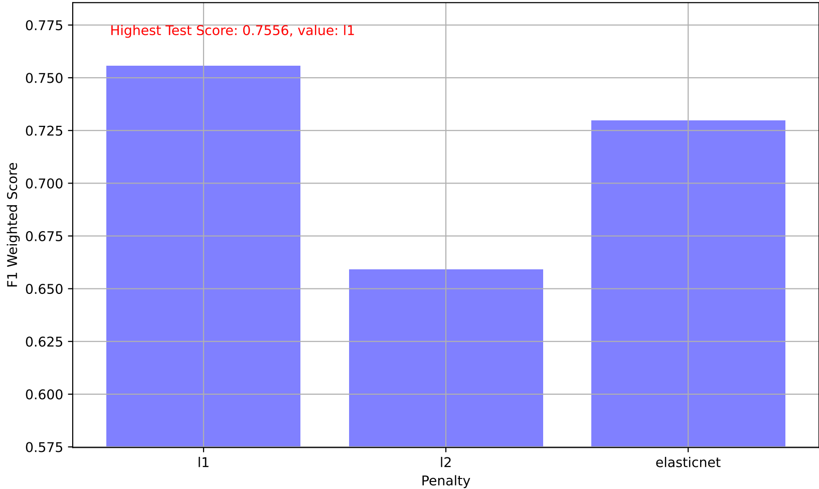
Perceptron - Penalty
