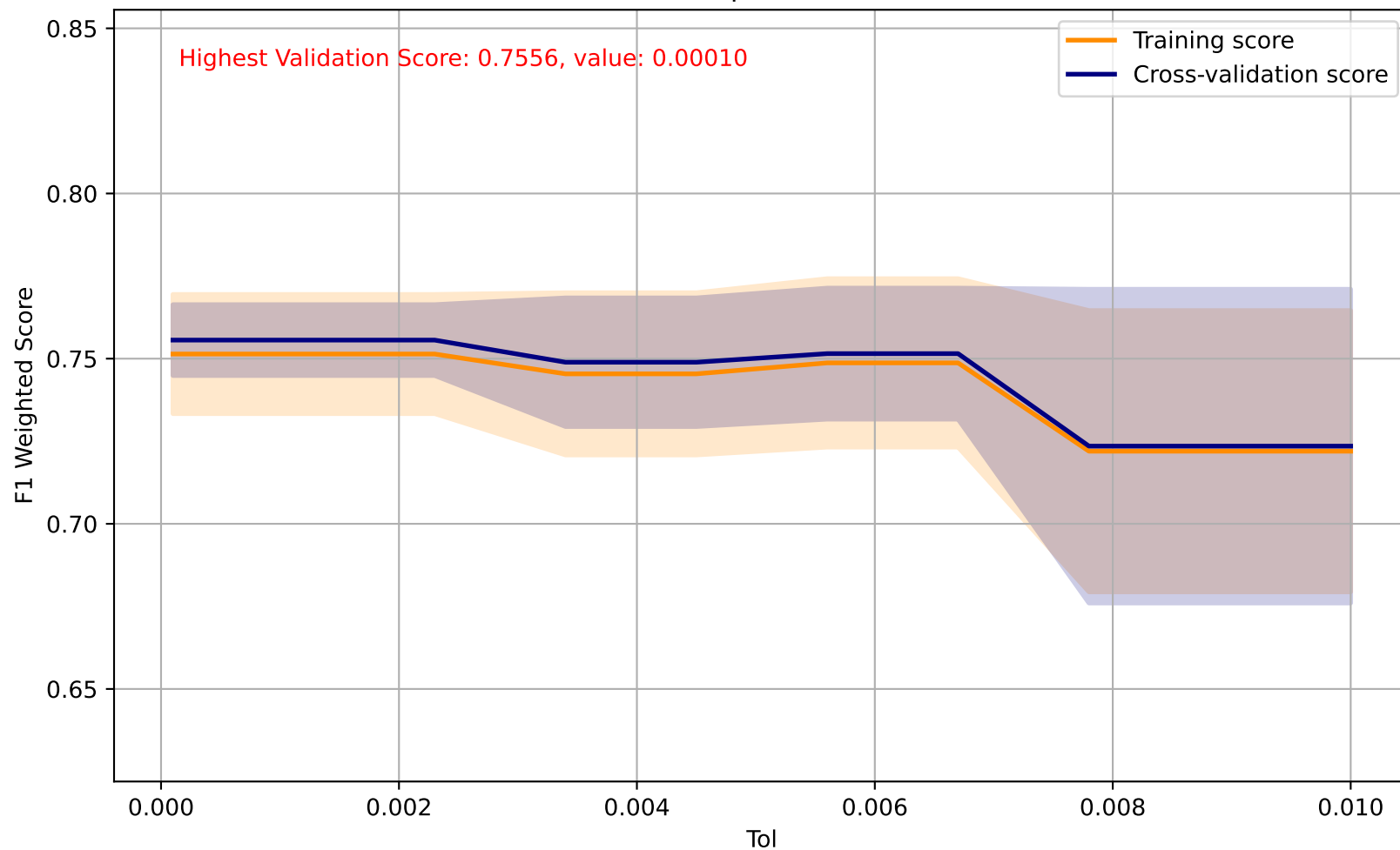
Perceptron - Tol
