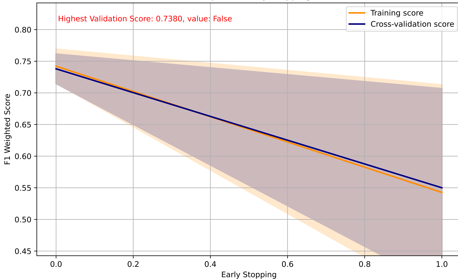
Perceptron - Early Stopping
