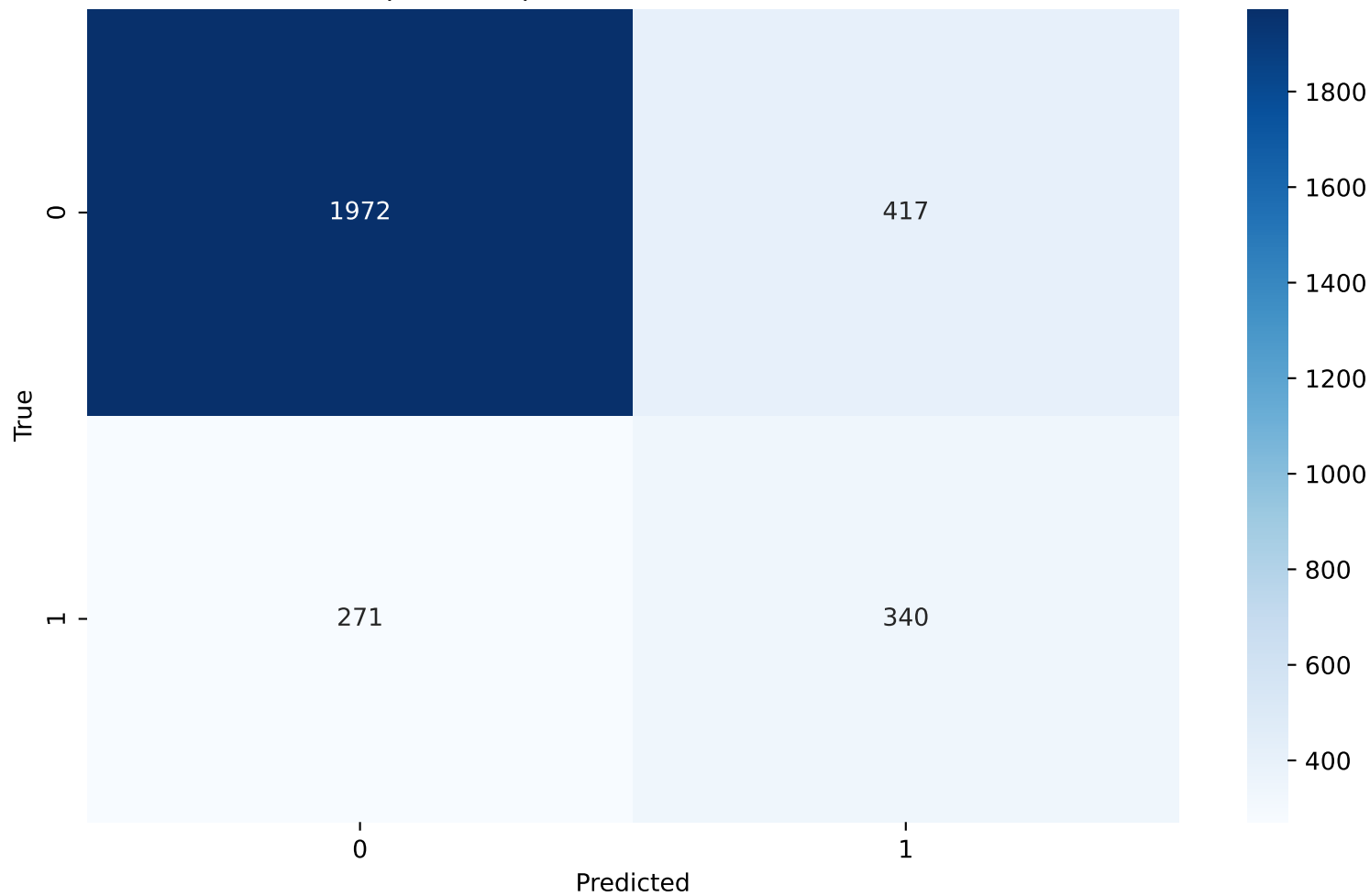
Perceptron - Alpha - Confusion Matrix(0.001)
