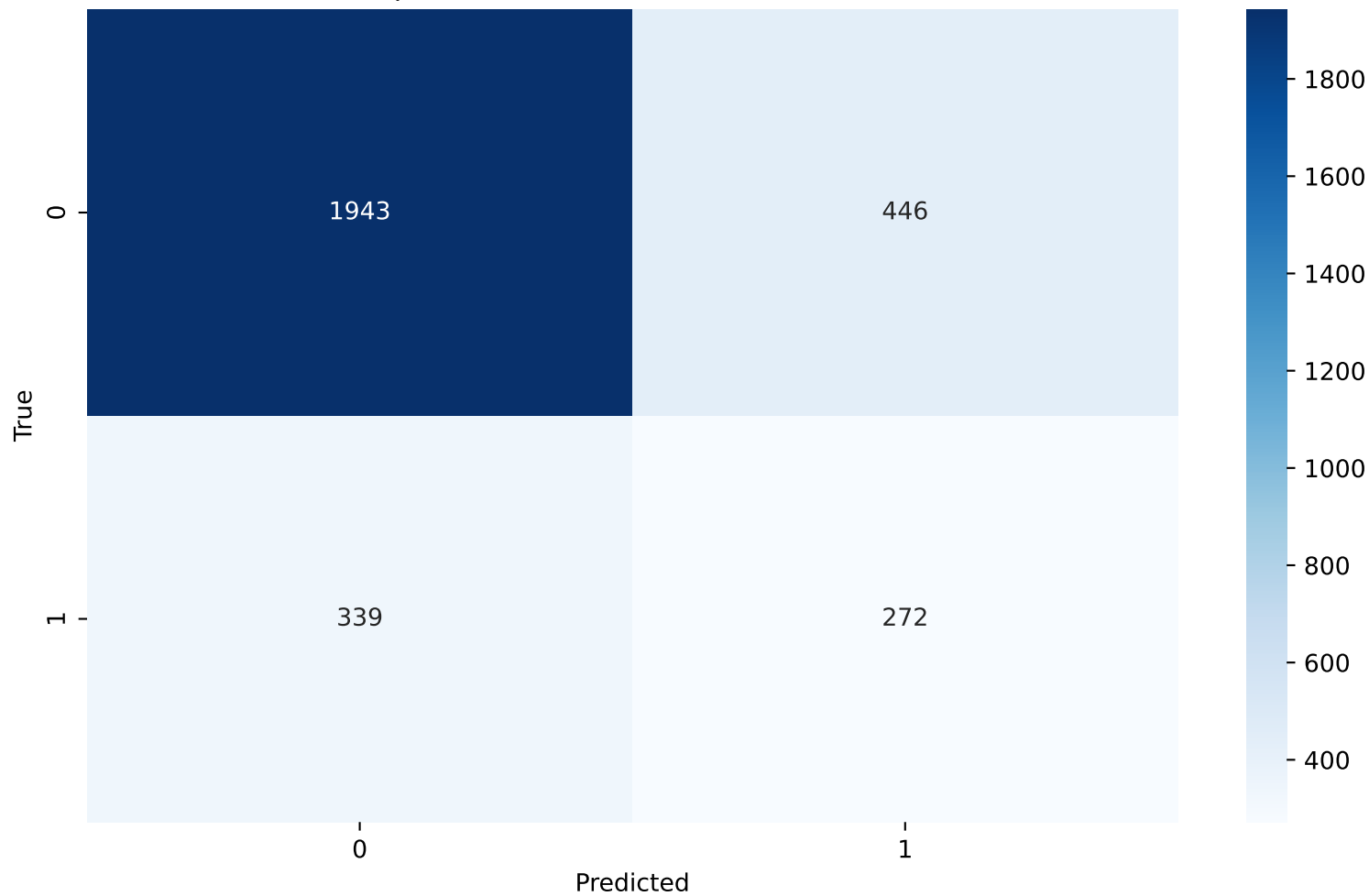
Perceptron - Eta0 - Confusion Matrix(0.005)
