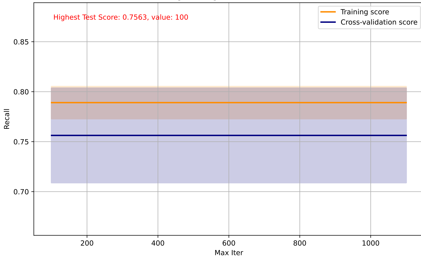
Logistic Regression - Max Iter
