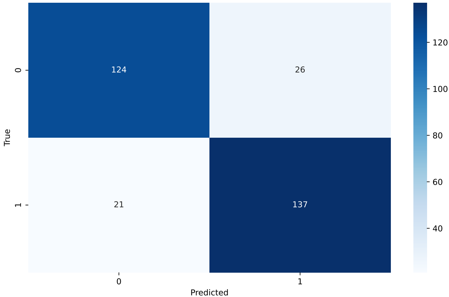
Logistic Regression - Confusion Matrix
