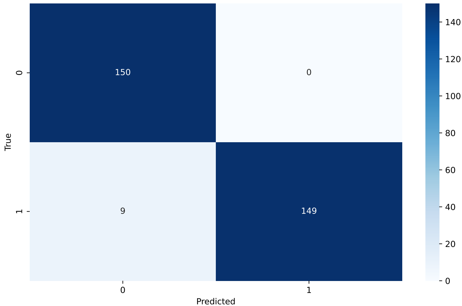
Decision Tree - Confusion Matrix
