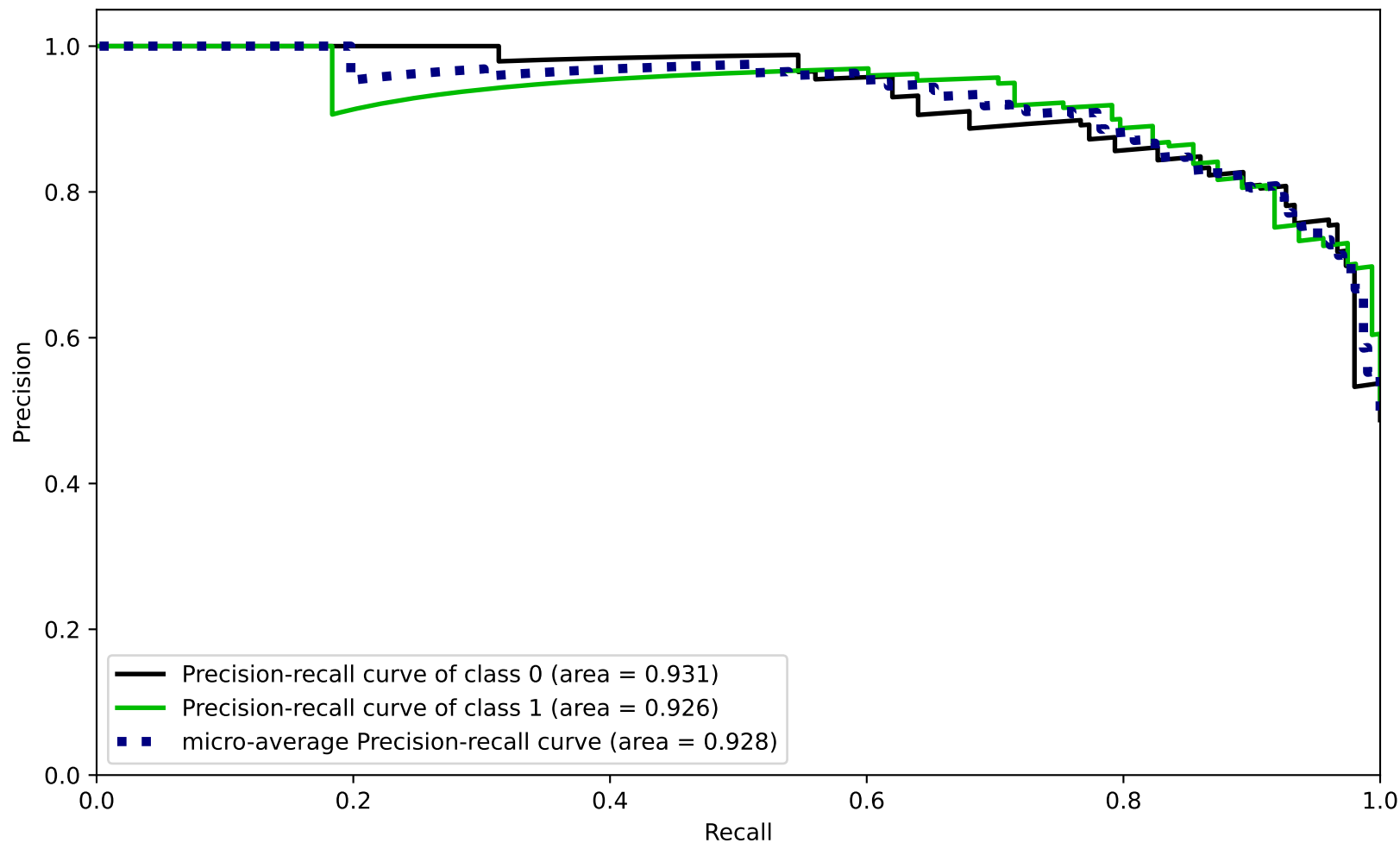
Precision-Recall Curve
