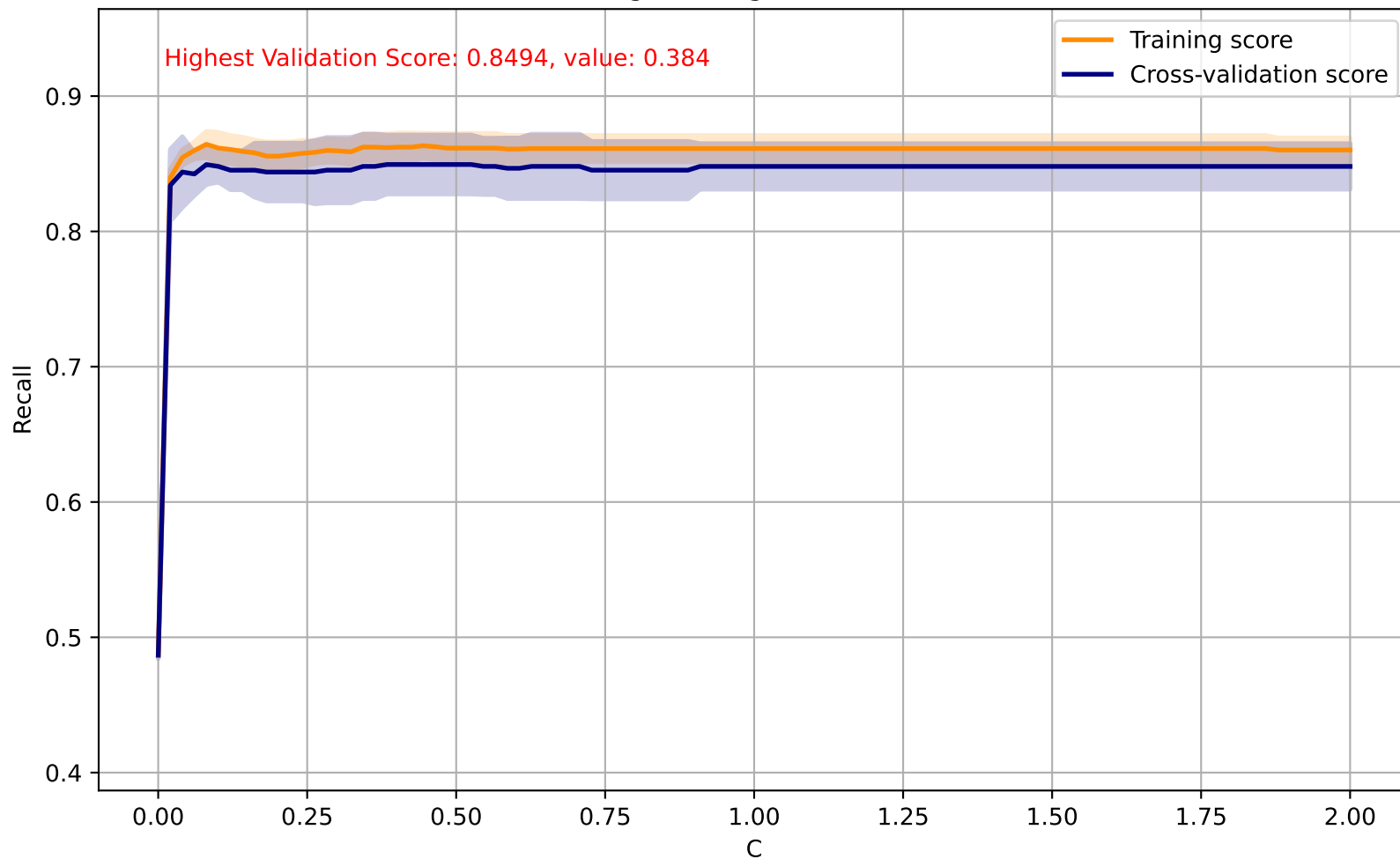
Logistic Regression - C
