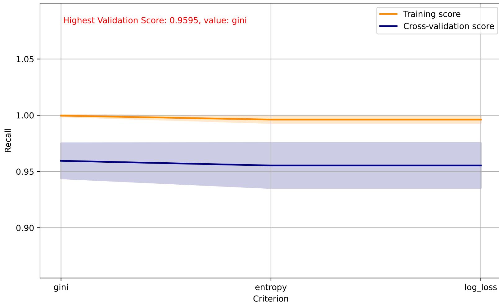
Decision Tree - Criterion
