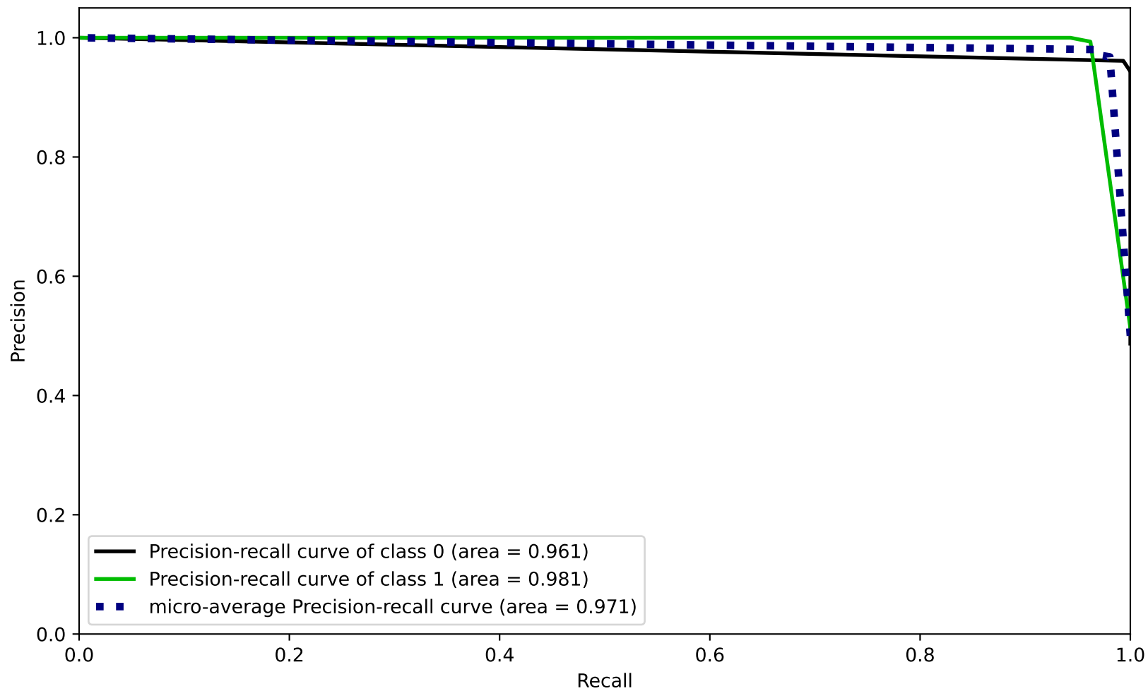
Precision-Recall Curve
