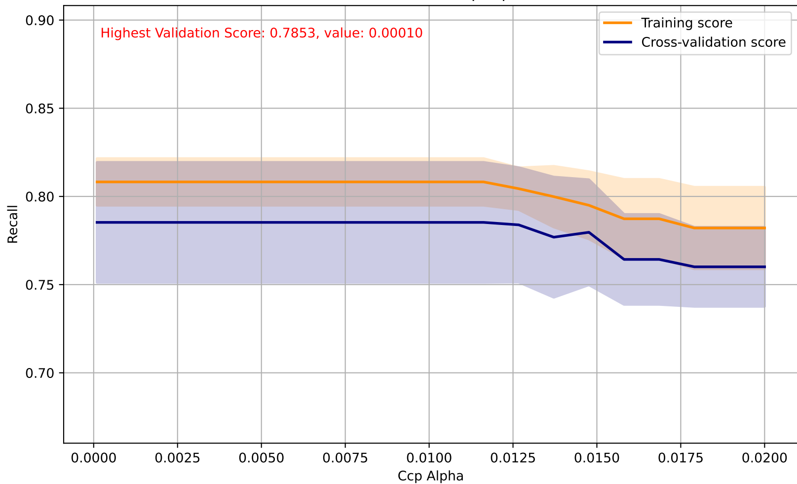
Decision Tree - Ccp Alpha
