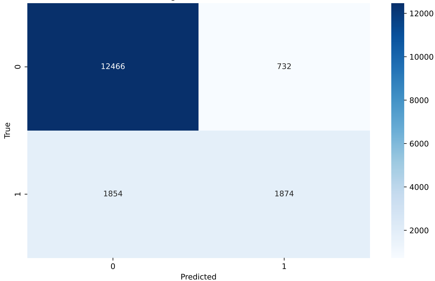
K-Nearest Neighbors - Confusion Matrix
