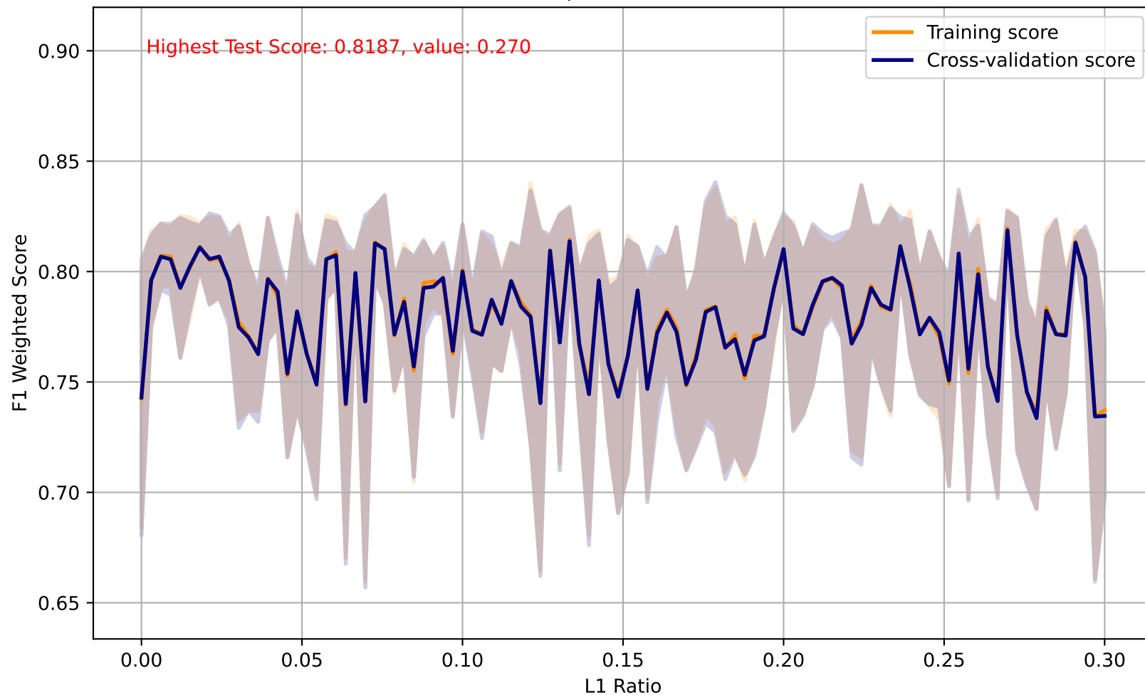
Perceptron - L1 Ratio
