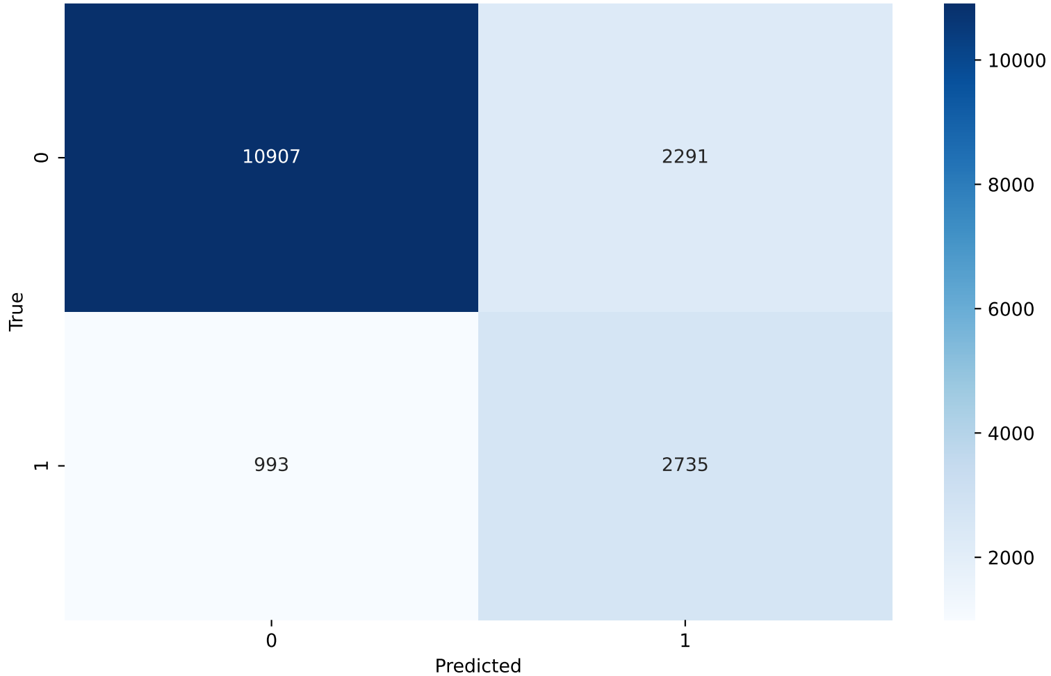
Perceptron - Confusion Matrix
