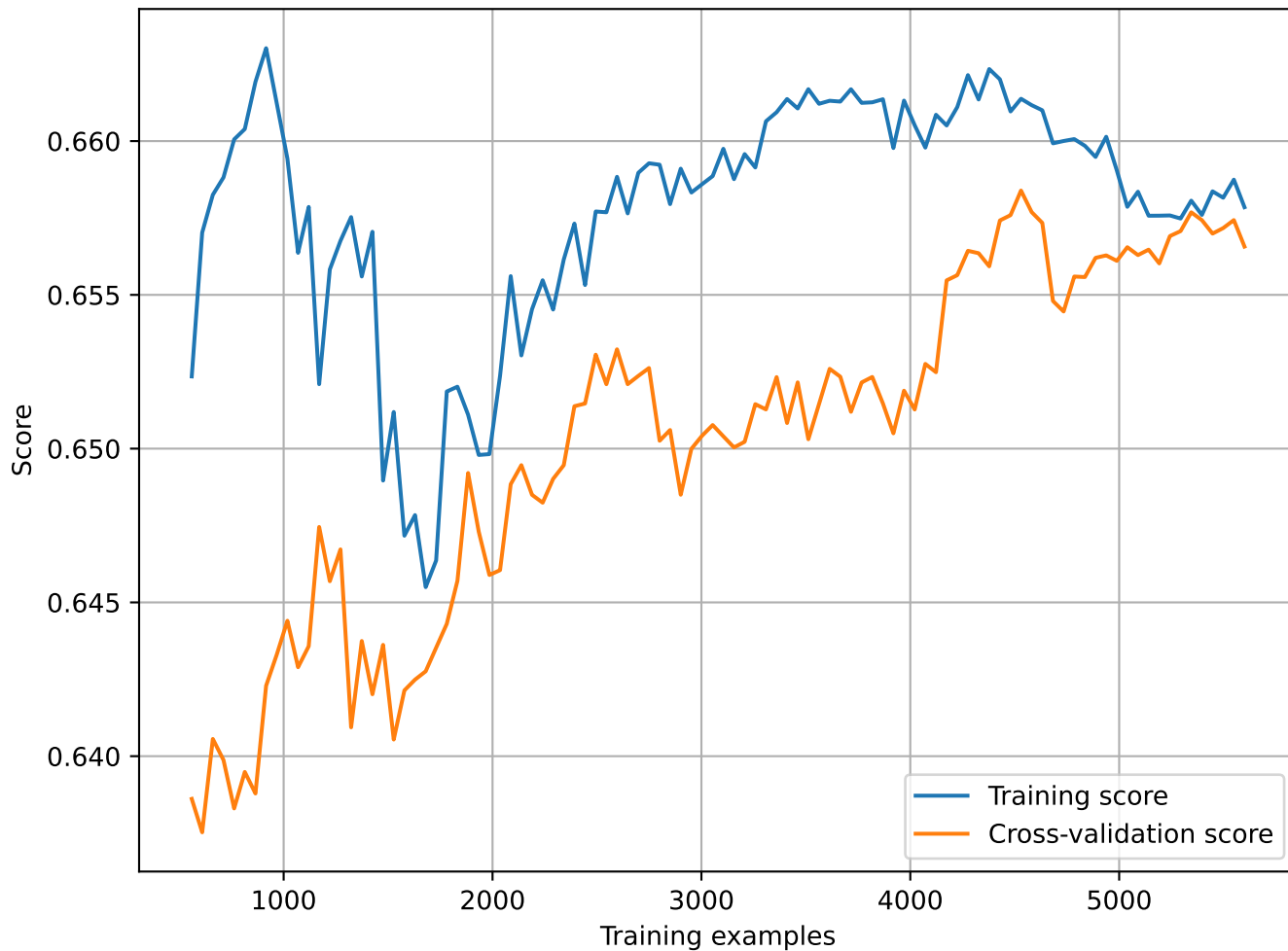
Learning Curve for Logistic Regression
