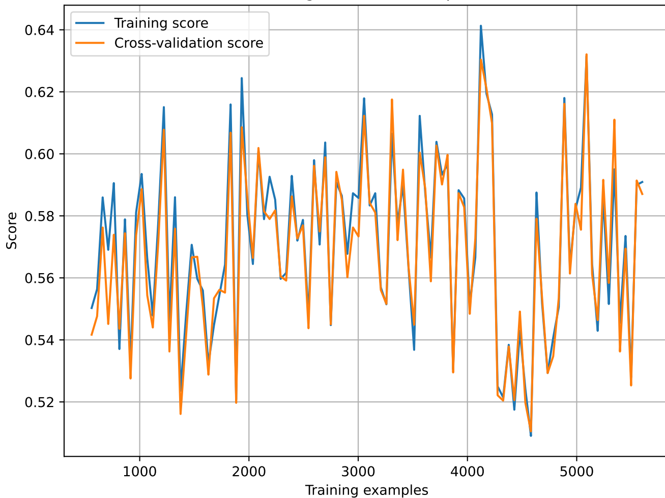
Learning Curve for Perceptron
