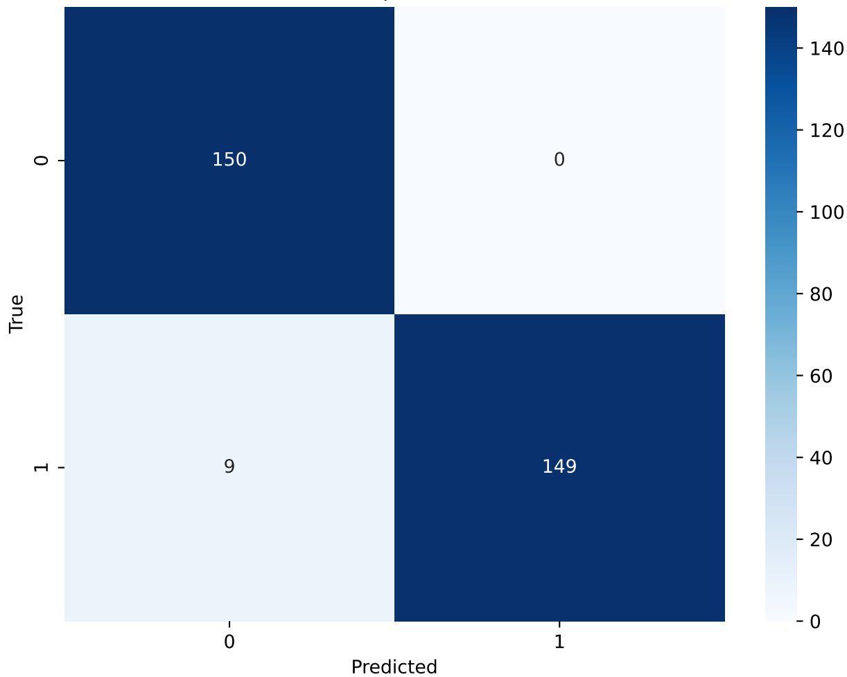
Decision Tree - Max Depth(9) - Confusion Matrix
