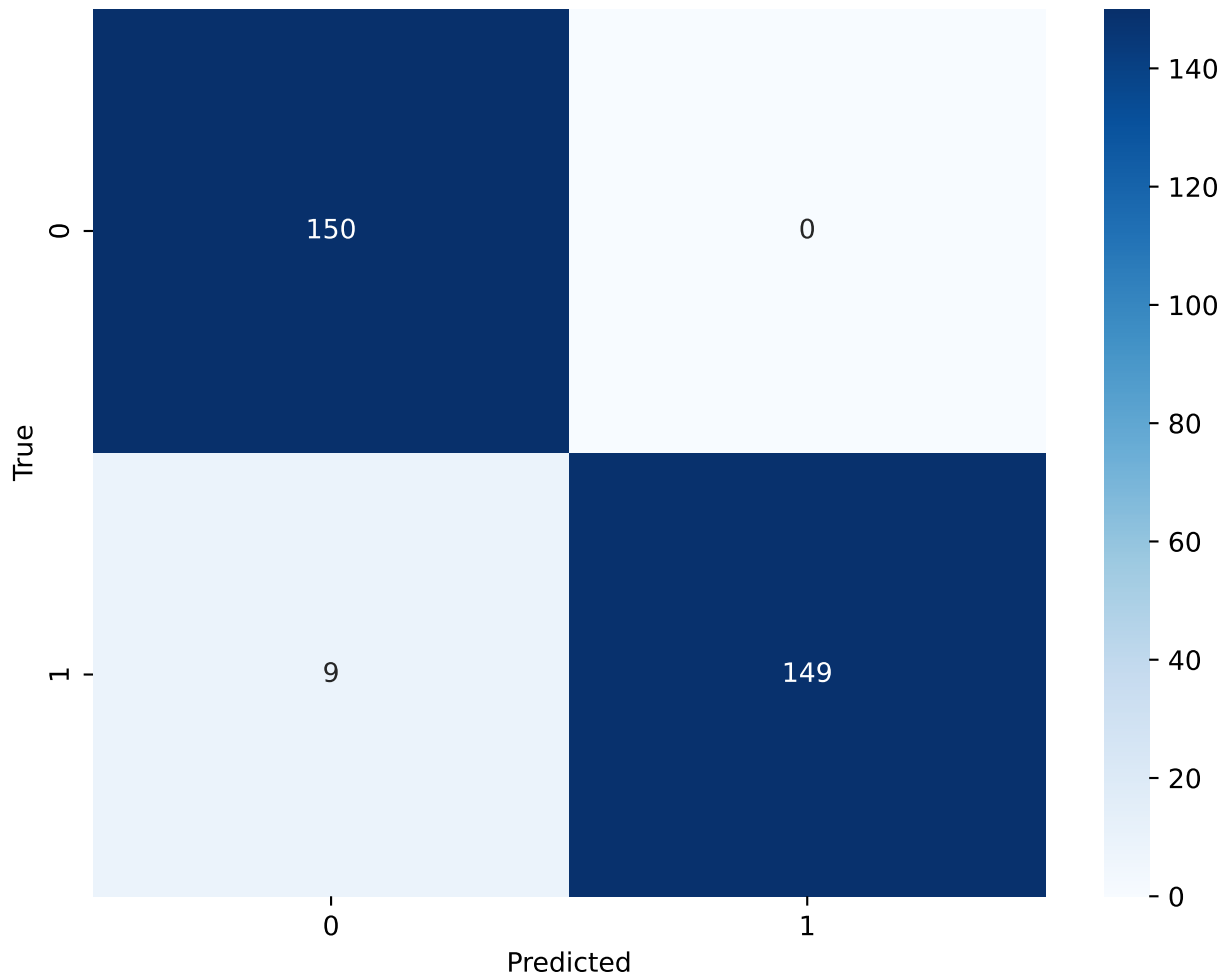
Decision Tree - Min Samples Leaf(1) - Confusion Matrix
