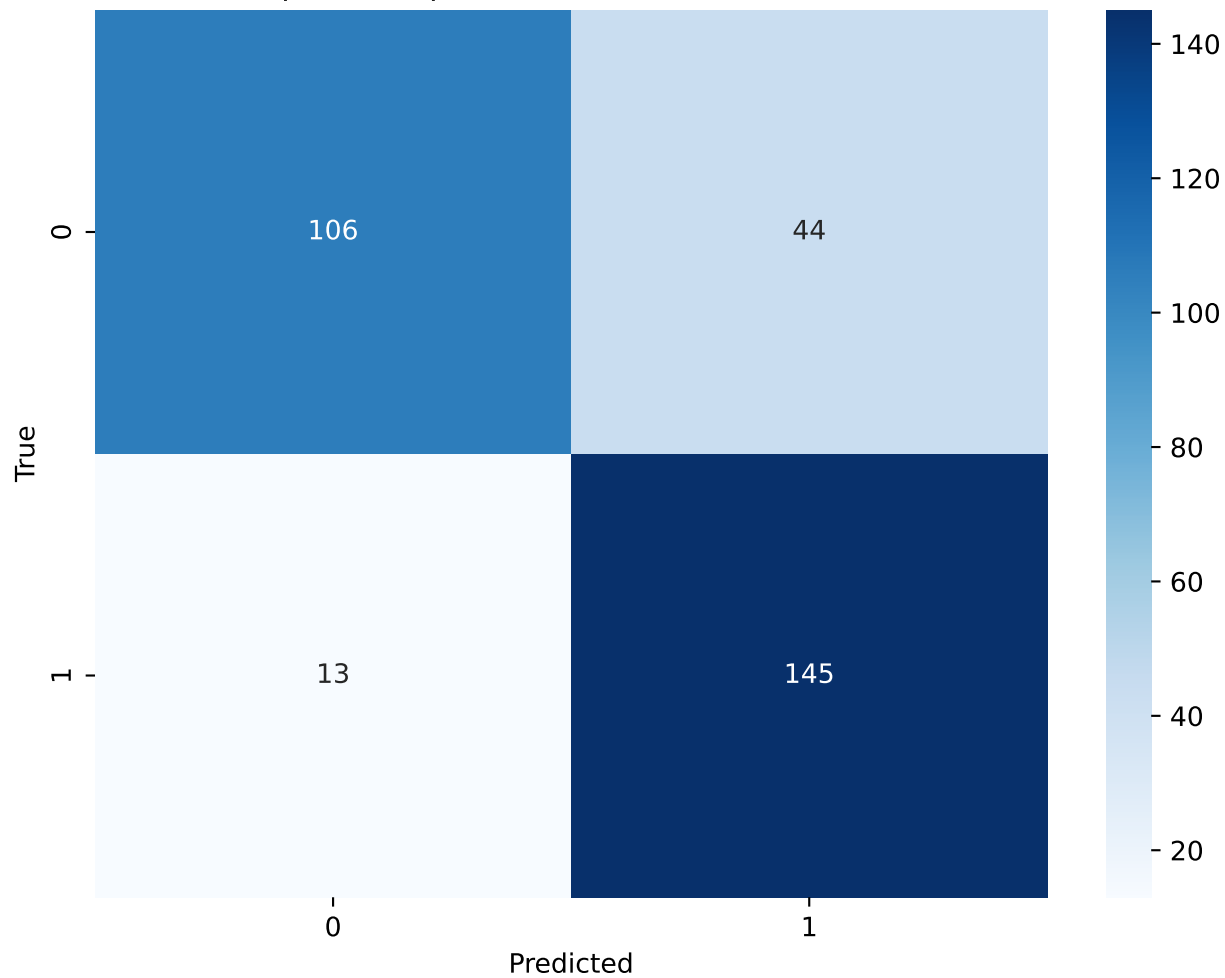
Perceptron - Alpha(0.00000) - Confusion Matrix
