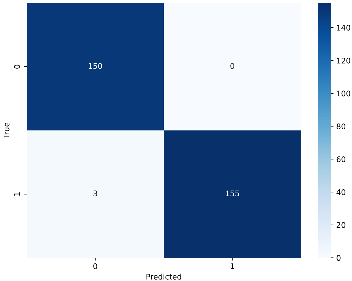
K-Nearest Neighbors - P(3) - Confusion Matrix
