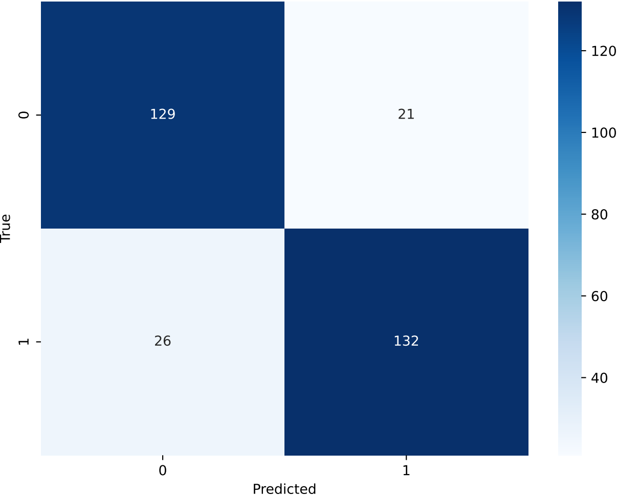
Logistic Regression - Class Weight(0:0.56 , 1:0.44) - Confusion Matrix
