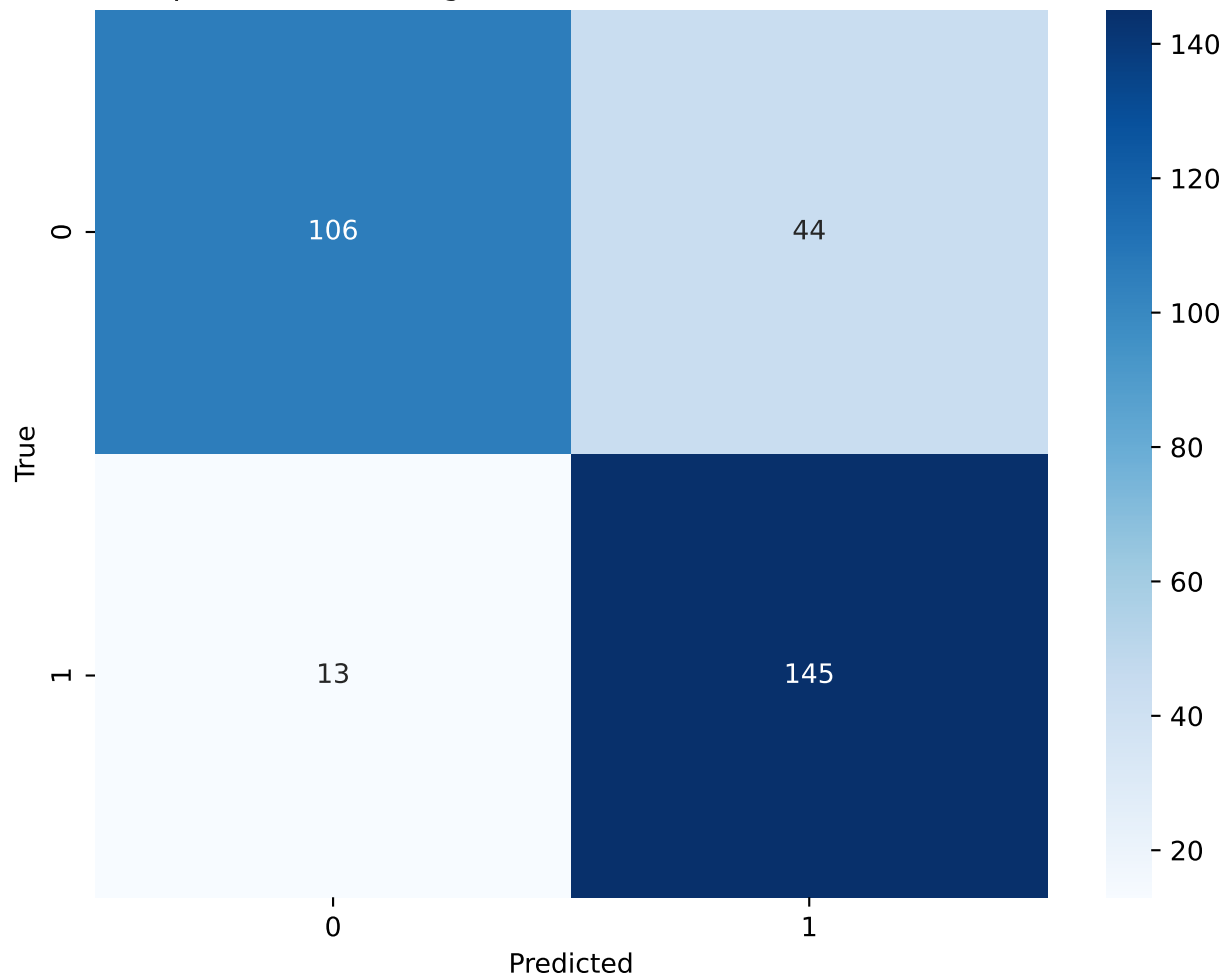
Perceptron - Class Weight(0:0.33 , 1:0.67) - Confusion Matrix
