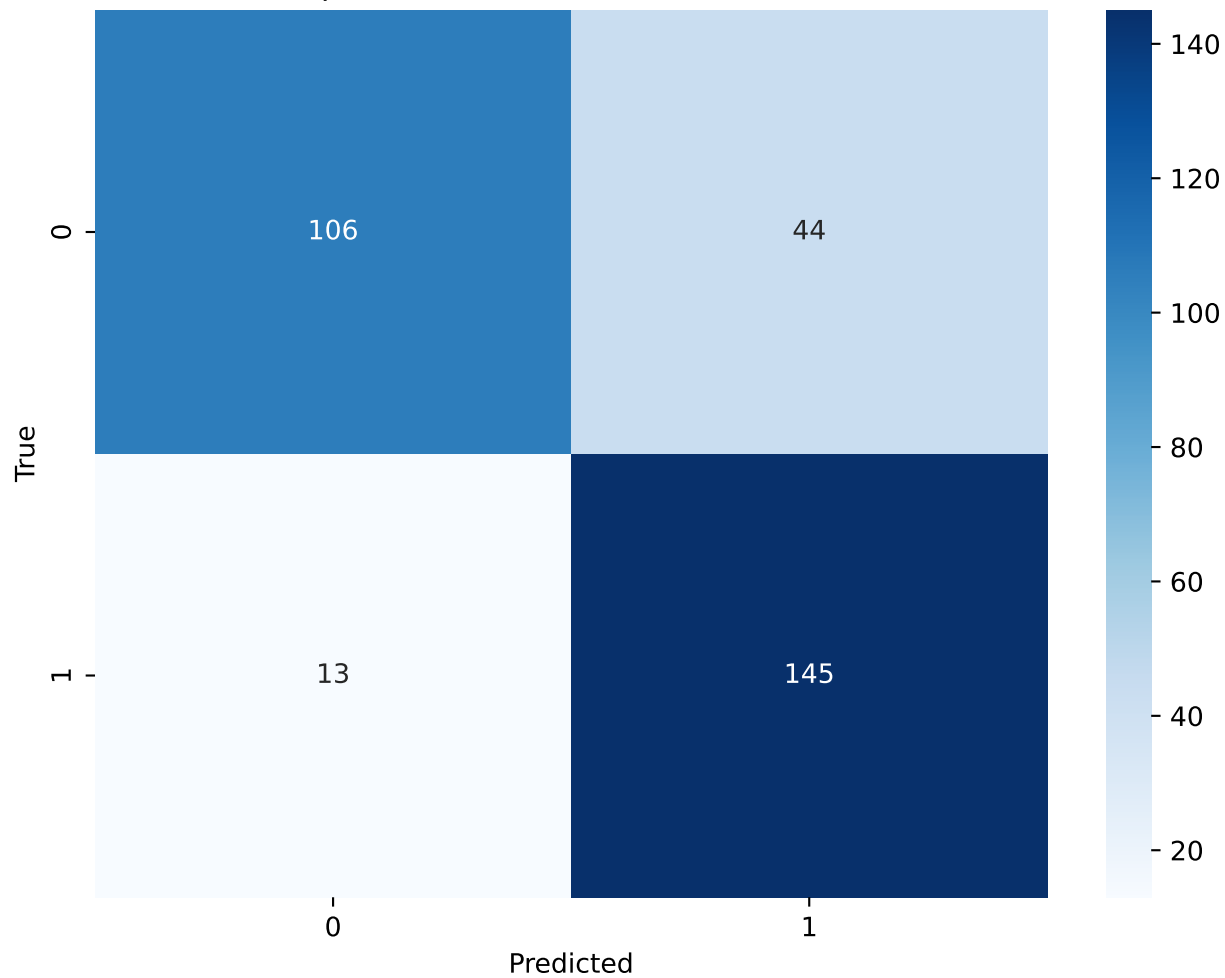
Perceptron - Eta0(0.03) - Confusion Matrix
