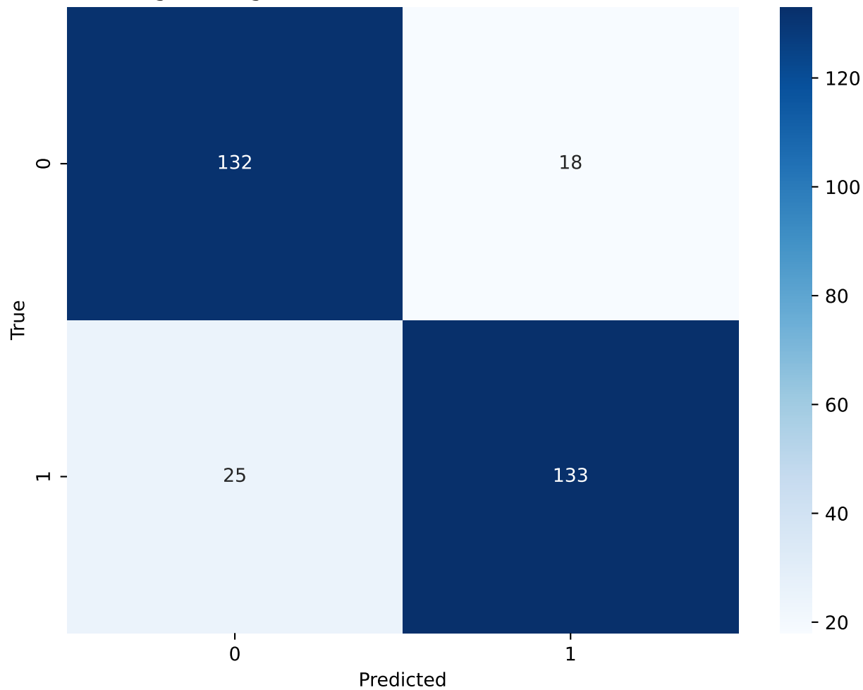
Logistic Regression - C(0.101) - Confusion Matrix
