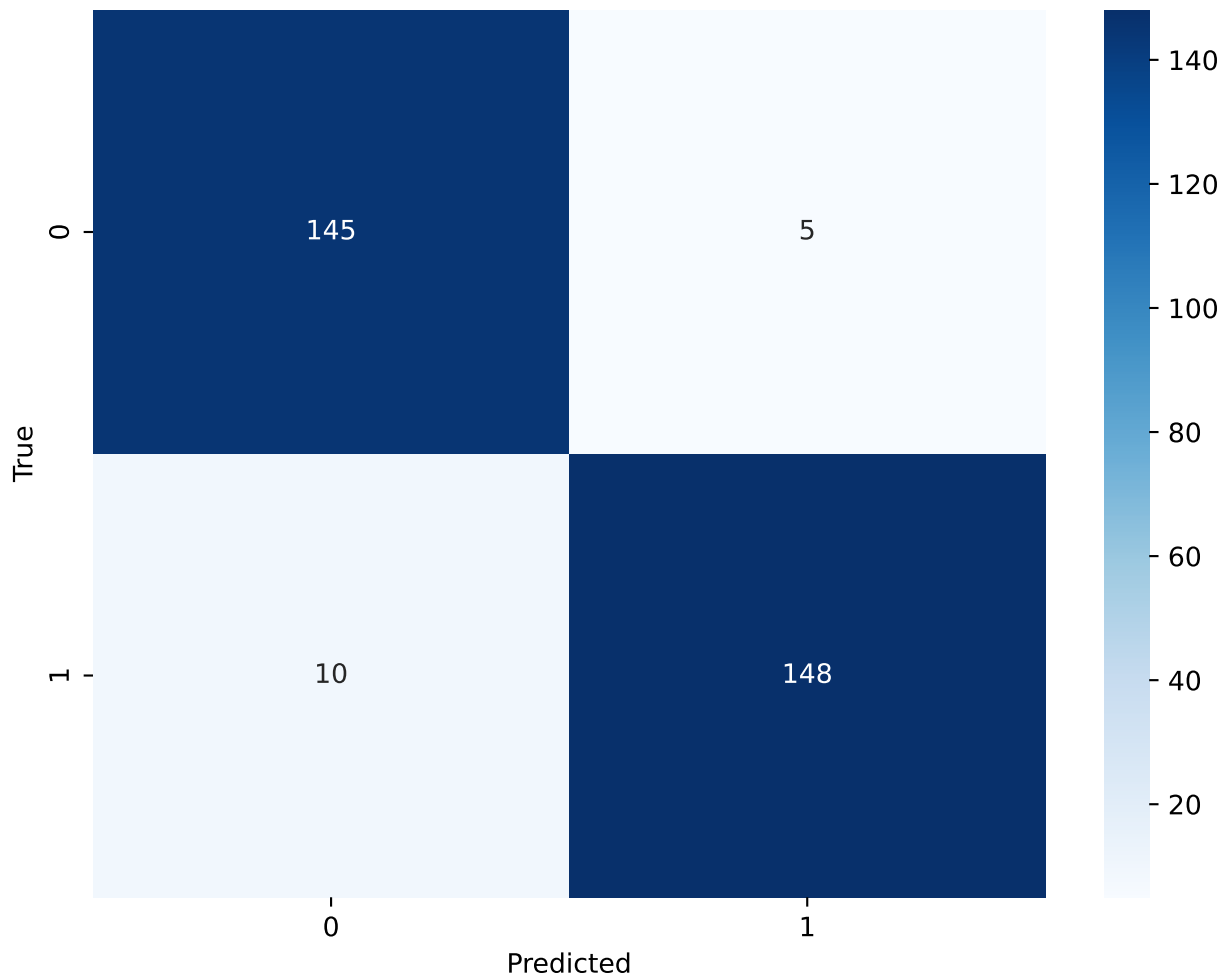
Decision Tree - Max Features(0.4) - Confusion Matrix
