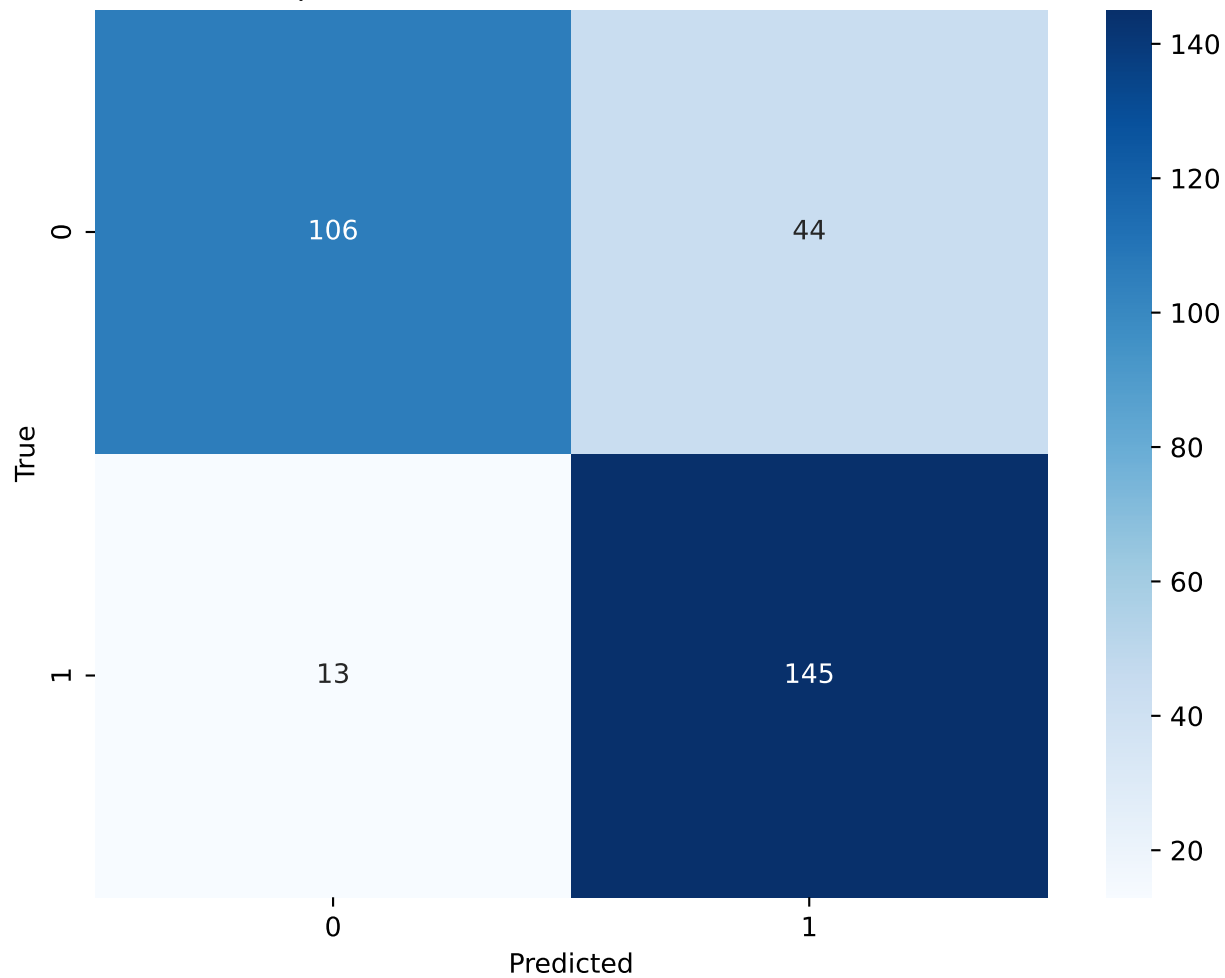
Perceptron - Max Iter(100) - Confusion Matrix
