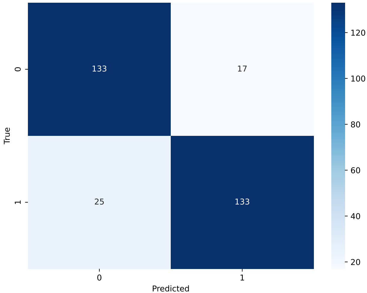
Logistic Regression - L1 Ratio(0.444) - Confusion Matrix
