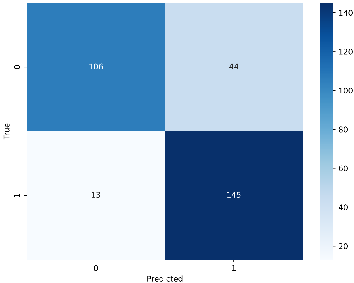
Perceptron - L1 Ratio(0.00000) - Confusion Matrix
