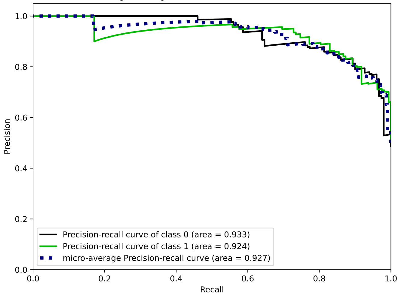
Logistic Regression - Precision-Recall Curve
