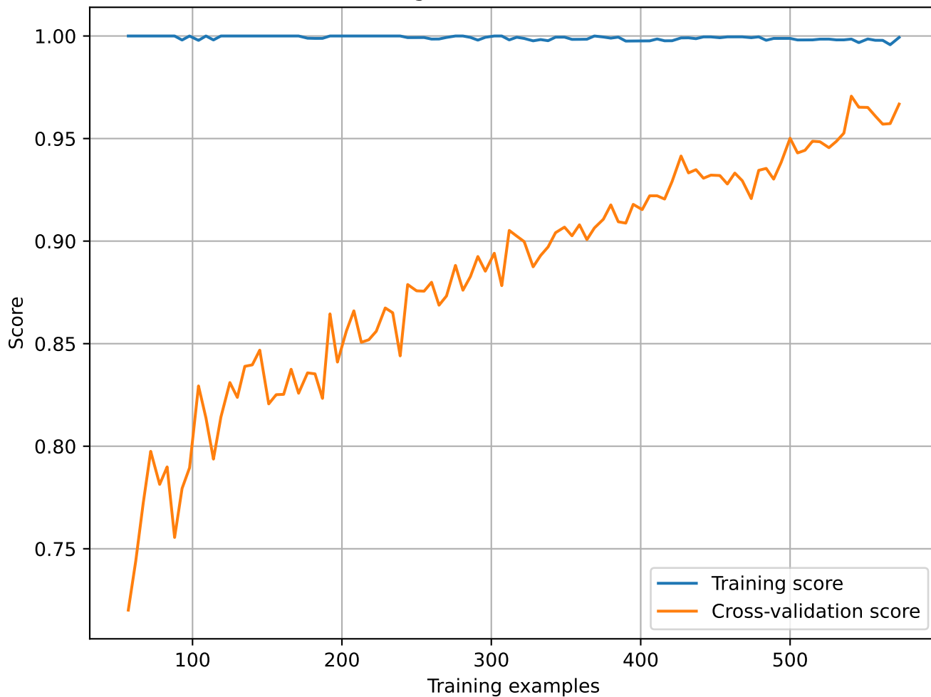
Learning Curve for Decision Tree
