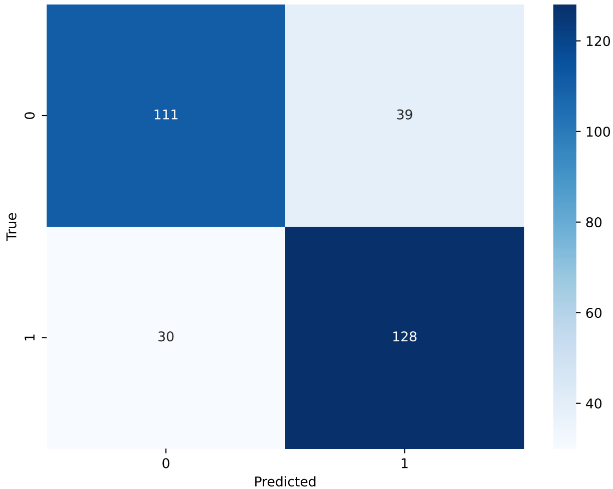
Perceptron - Confusion Matrix
