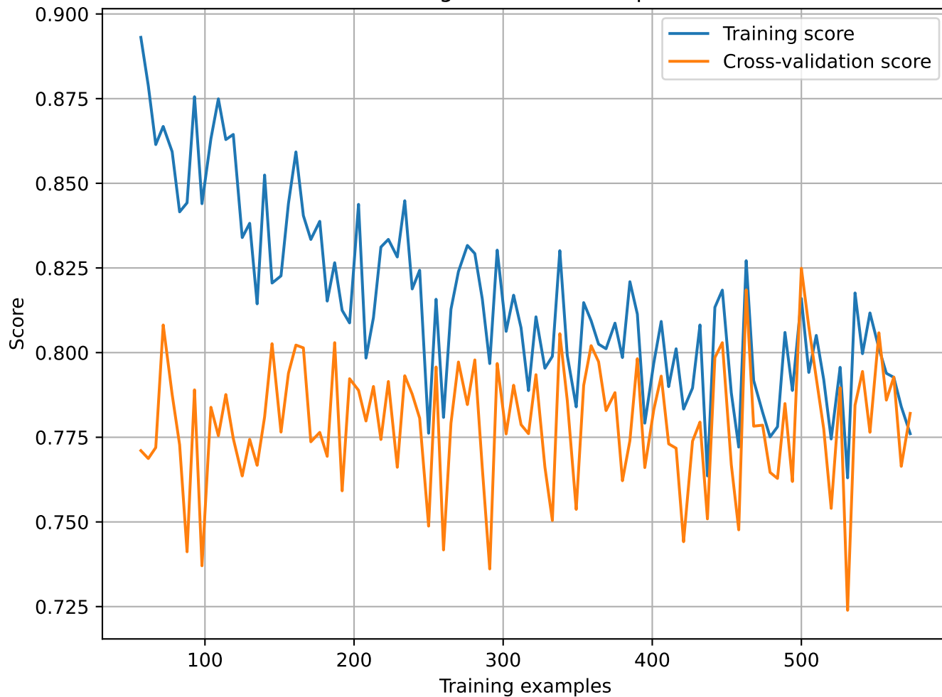
Learning Curve for Perceptron
