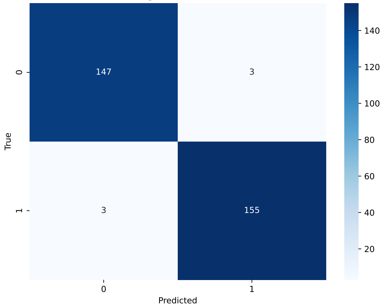
K-Nearest Neighbors - Confusion Matrix
