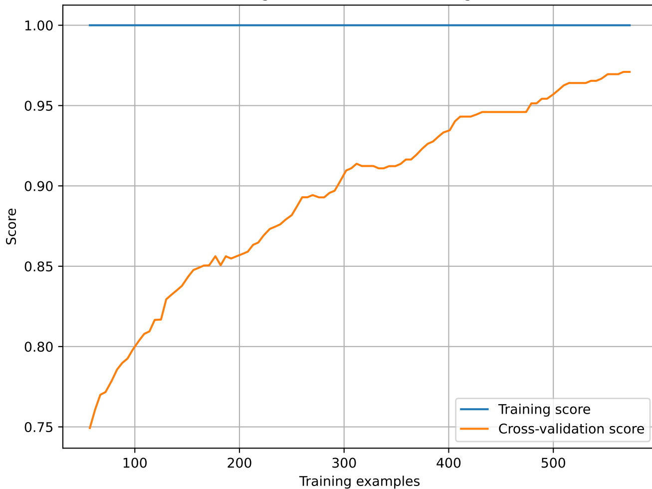
Learning Curve for K-Nearest Neighbors
