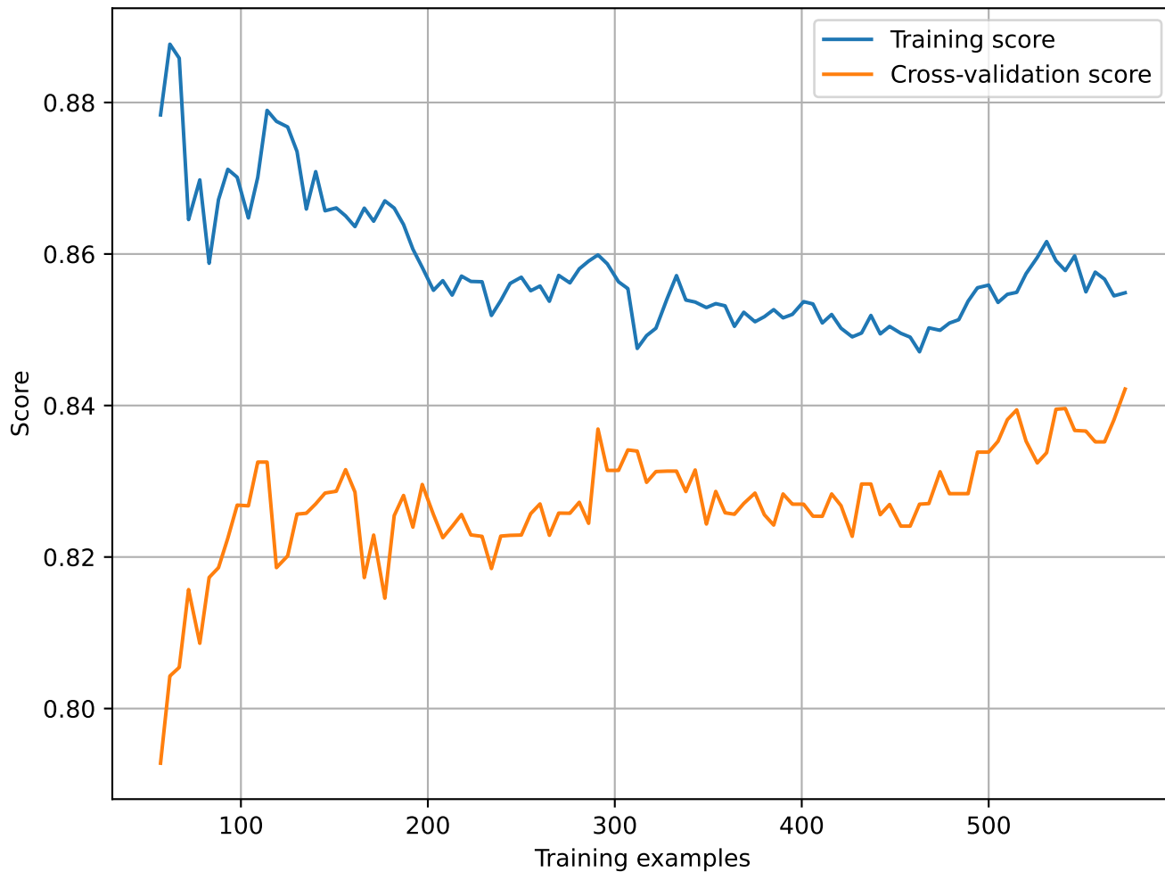
Learning Curve for Logistic Regression
