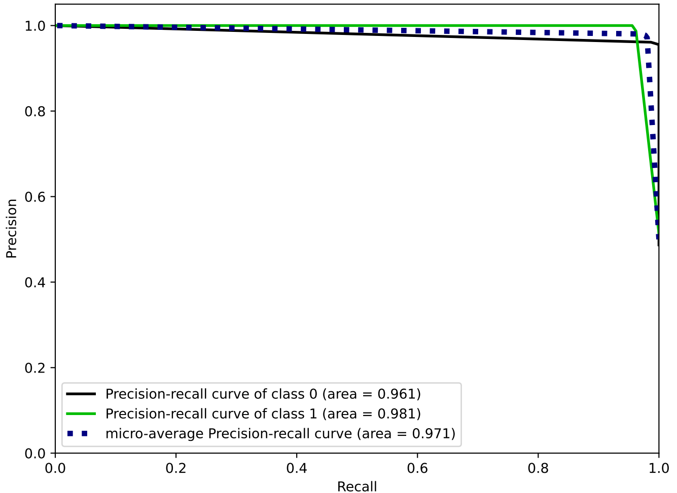
Decision Tree - Precision-Recall Curve
