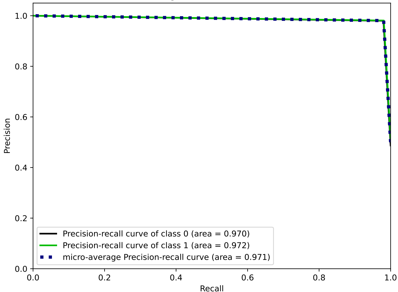
K-Nearest Neighbors - Precision-Recall Curve
