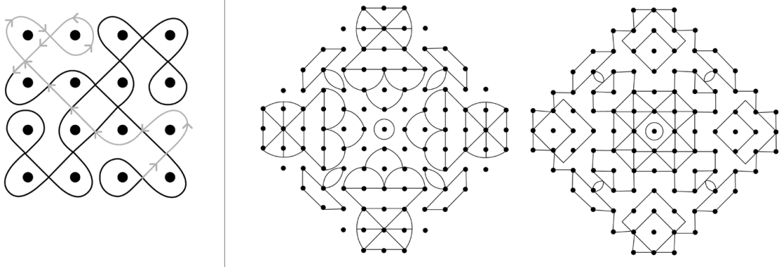
Figure 2 (Left) A Pulli Kolam drawing made on a 4x4 point lattice. (Right) Pulli Kolam variation: connect the points.
