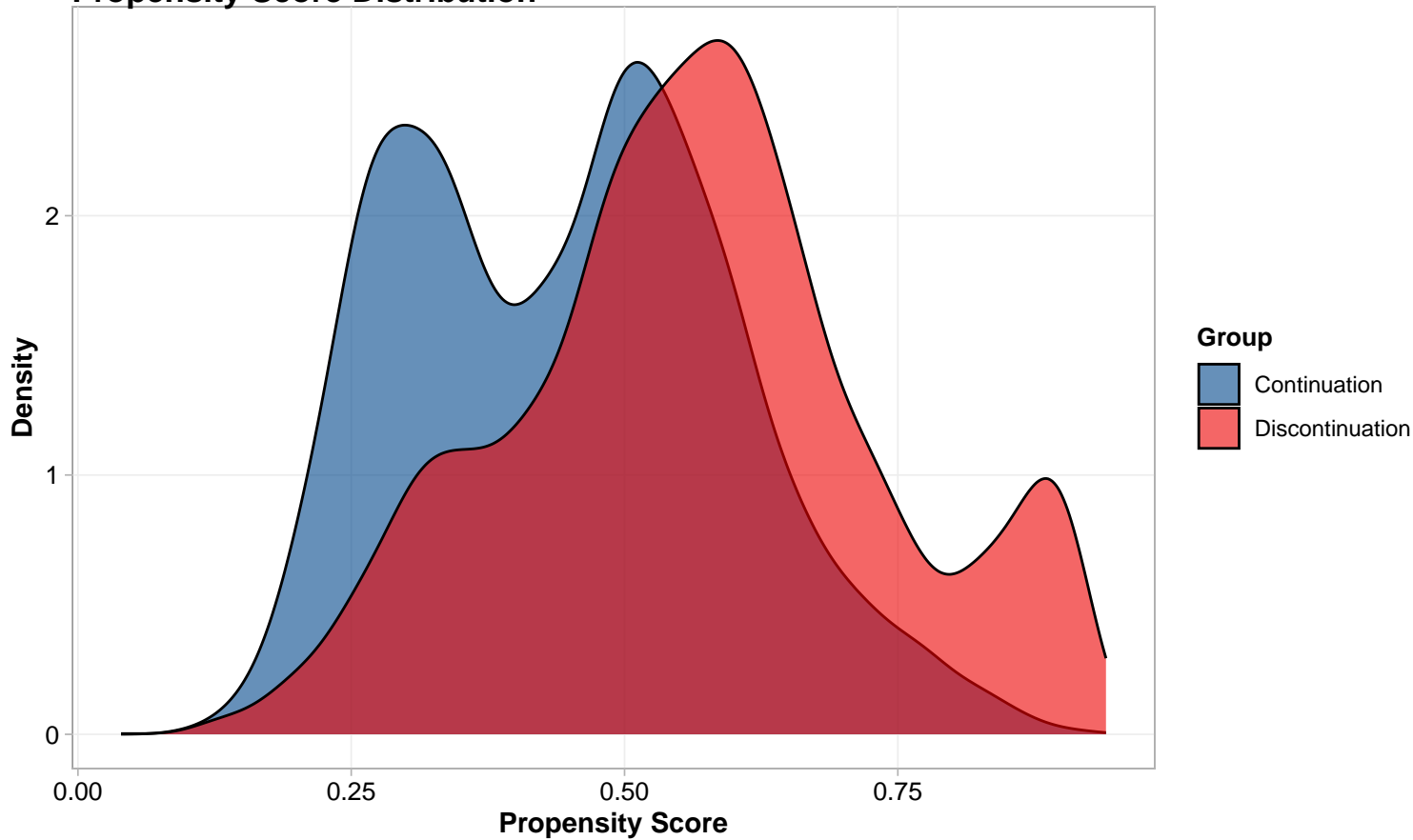
Propensity Score Distribution
