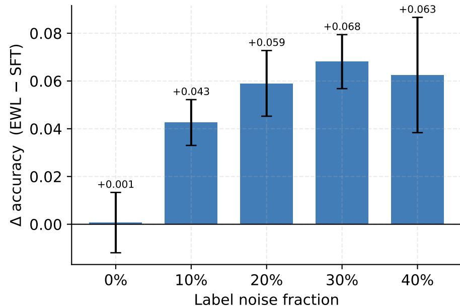
FGVC-Aircraft
