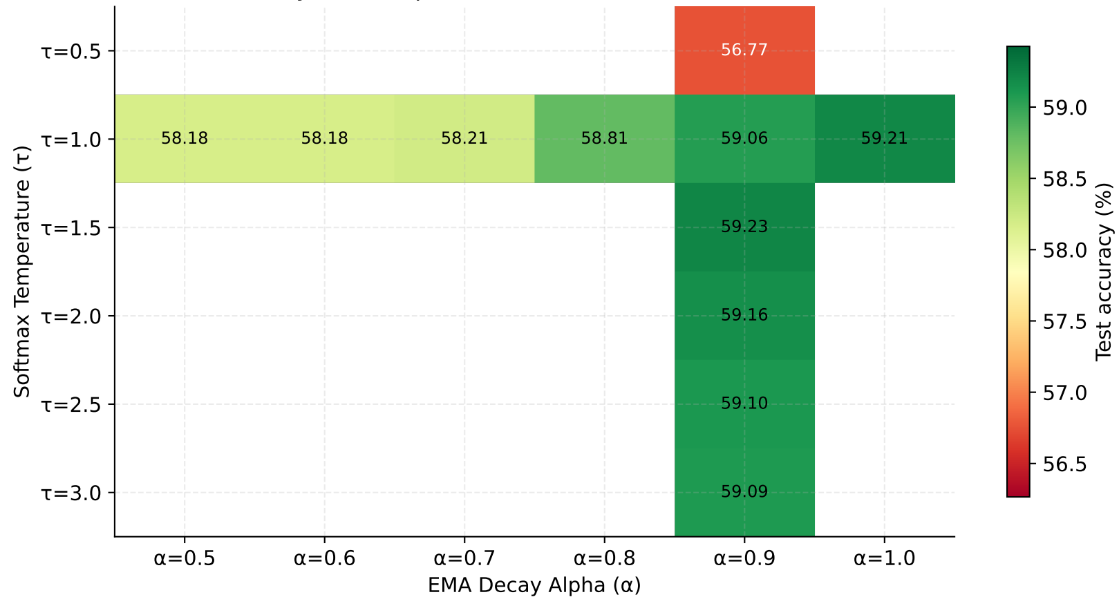
EWL Test Accuracy Heatmap (rank=4, FGVC-Aircraft, mean over 3 seeds)
