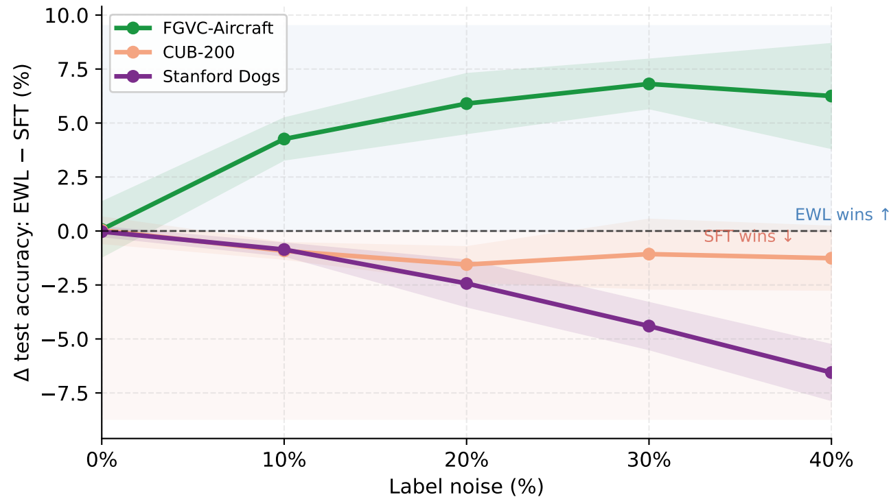
EWL advantage vs noise — per dataset (above zero = EWL wins; below zero = SFT wins)
