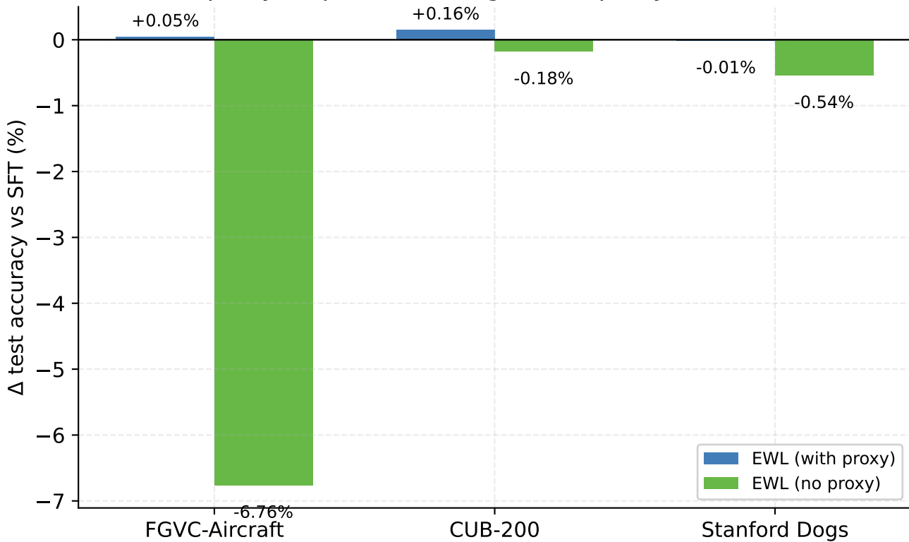
EWL vs EWL-no-proxy: impact of LoRA gradient proxy (rank=4, \alpha=0.9 , \tau=1.0 )
