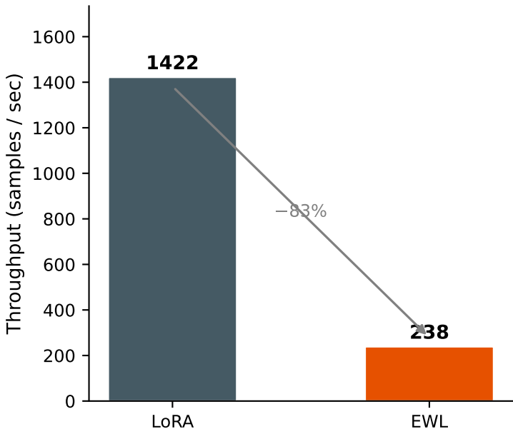
Training throughput: LoRA vs EWL
