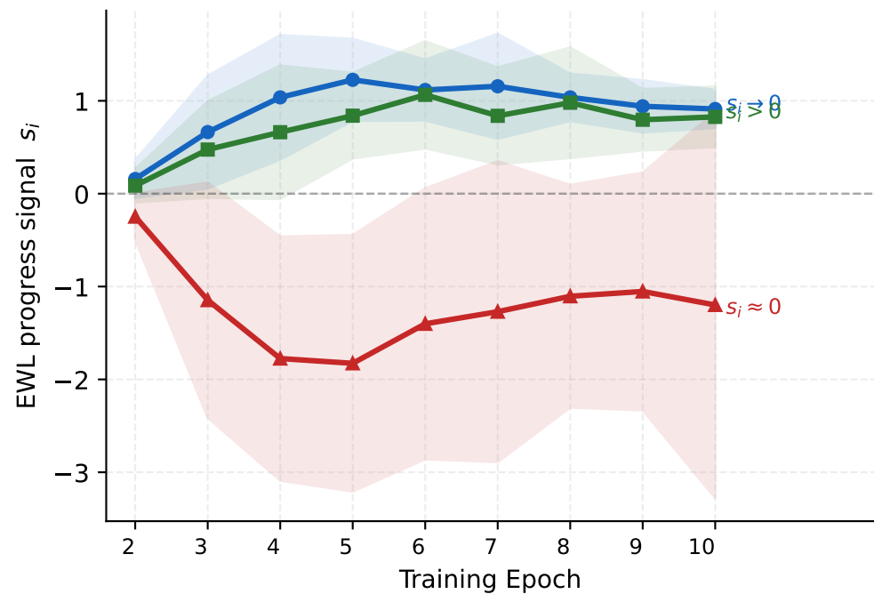
(b) EWL progress signal s_i per category
