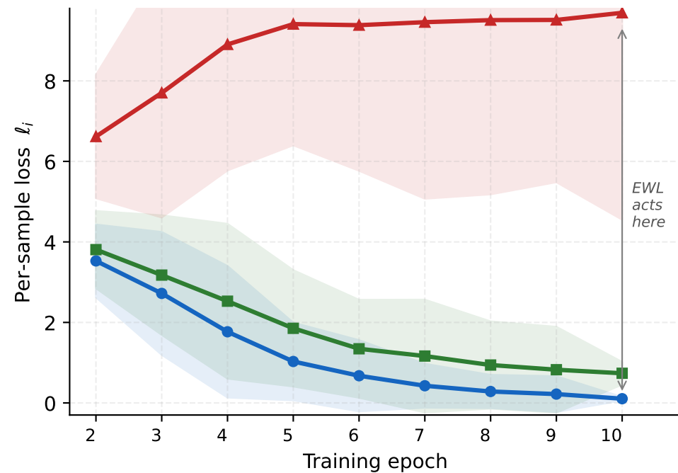
(a) Loss trajectories — three sample categories
