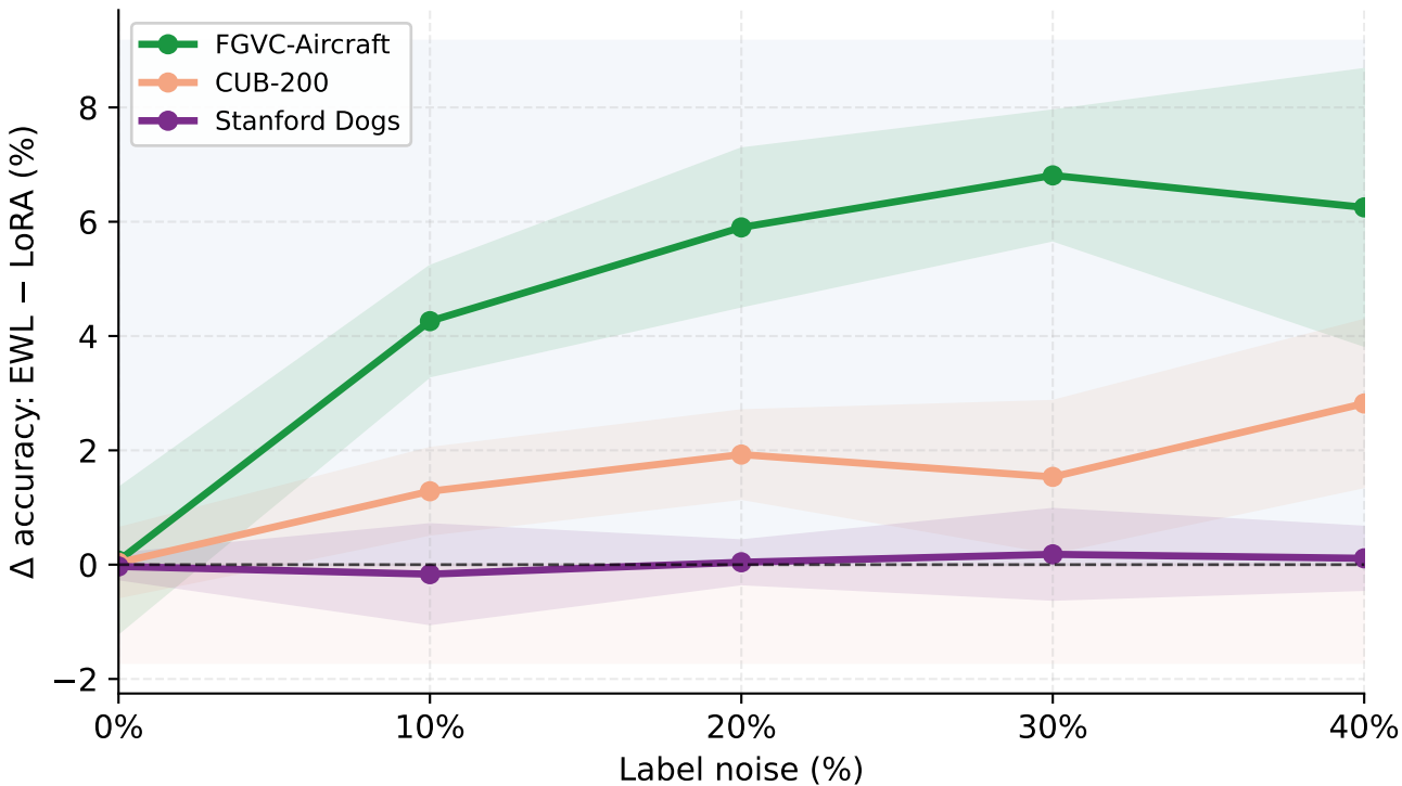
EWL advantage vs noise — per dataset (above zero = EWL wins; below zero = LoRA wins)
