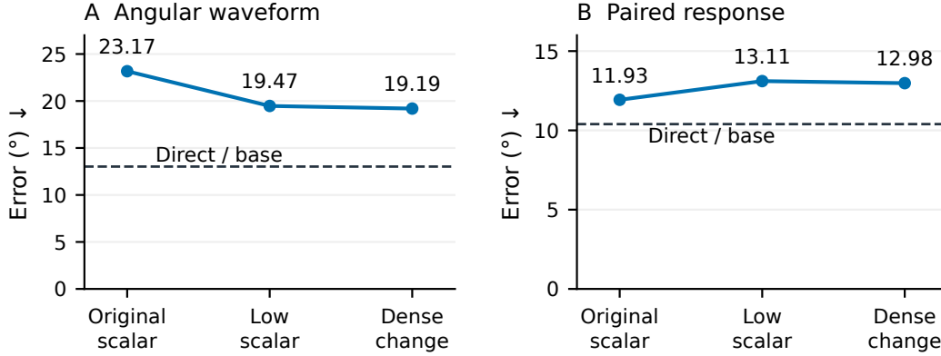
Figure 5: Does dense supervision improve on a lower scalar weight? Delta JEPA readout means on ViTPose only, over the same 14 development people and three seeds. Original scalar, low scalar, and dense retain the same geometry term; the horizontal direct/base reference omits it. The low-scalar and dense arms are the matched repair comparison. Waveform recovery accompanies higher response error than the original scalar arm. All axes start at zero and all means include failure penalties. Intervals for the primary contrast appear in Figure 4; no intervals are implied for these means.
