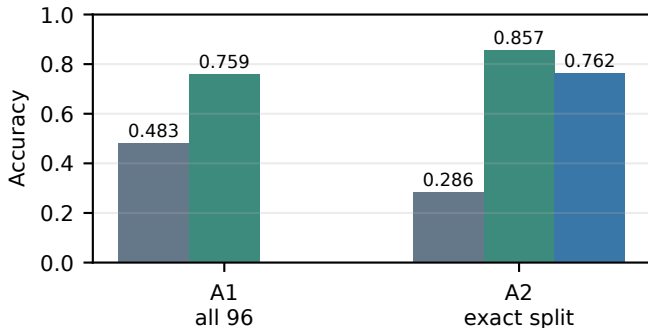
Mean accuracy across grouped folds
