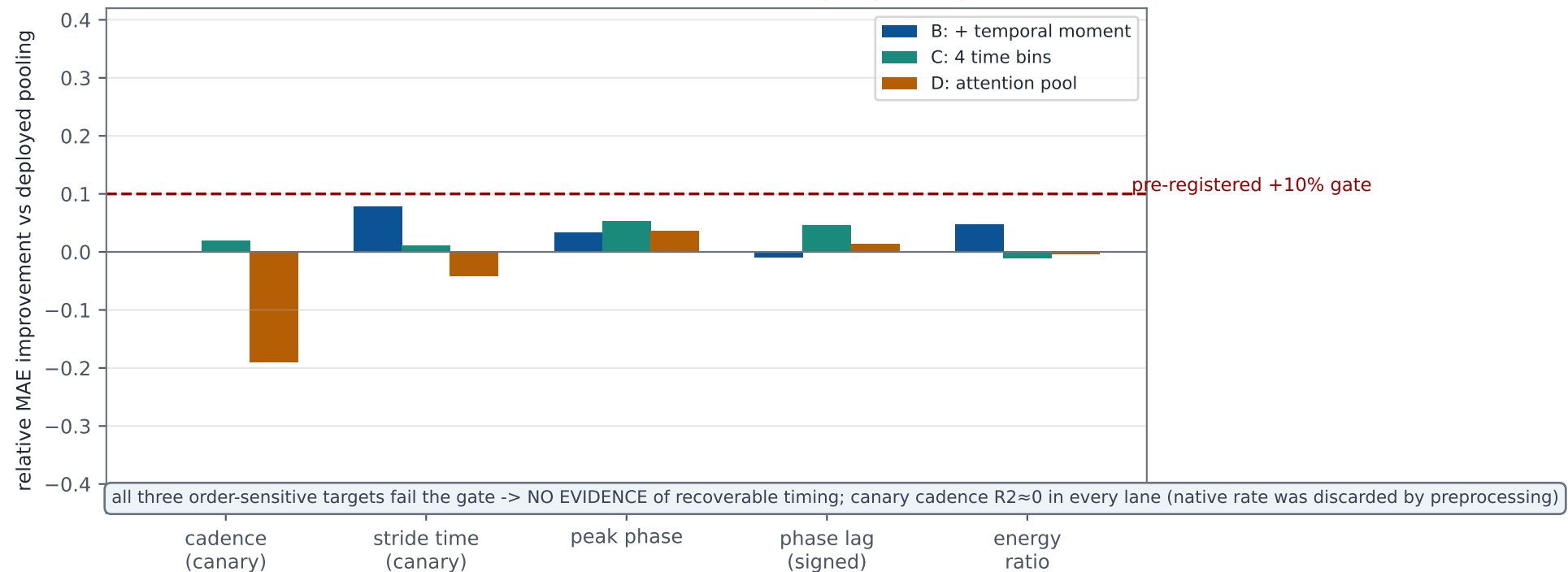
Same frozen tokens, different readouts (source-grouped ridge)
