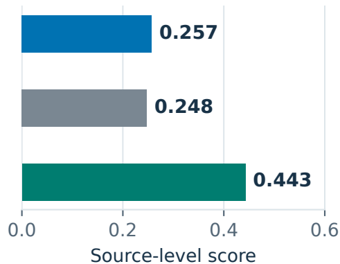
Balanced accuracy
