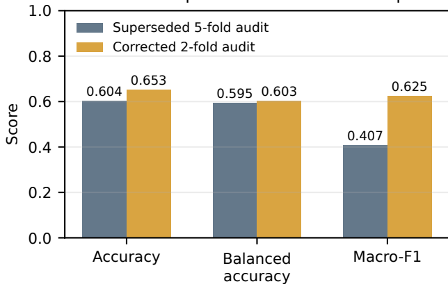
Evaluation repair with the same checkpoint
