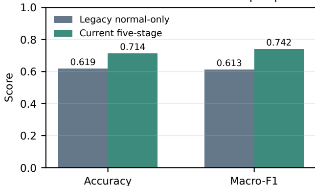
Model revision on the exact exp5 split
