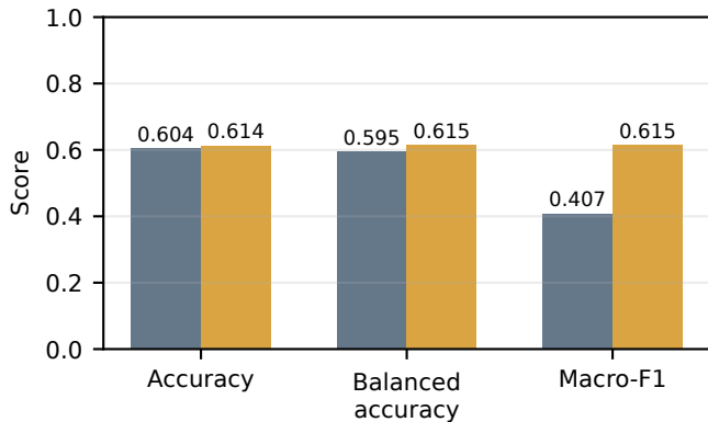
Evaluation repair with the same checkpoint
