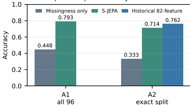
Sequence-split accuracy and controls
