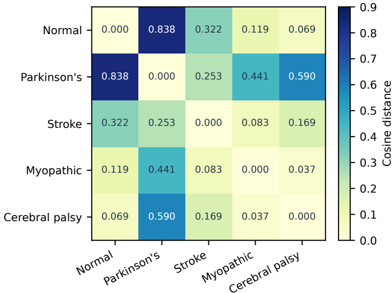
Canonical 96: cosine distance between condition centroids
