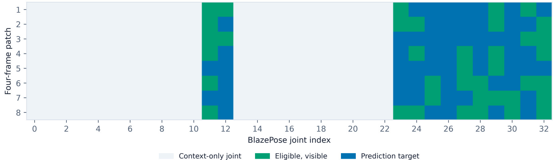
One deterministic illustration of a stochastic neurologic target mask
