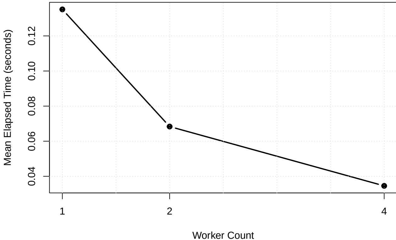
Mean Elapsed Time by Worker Count
