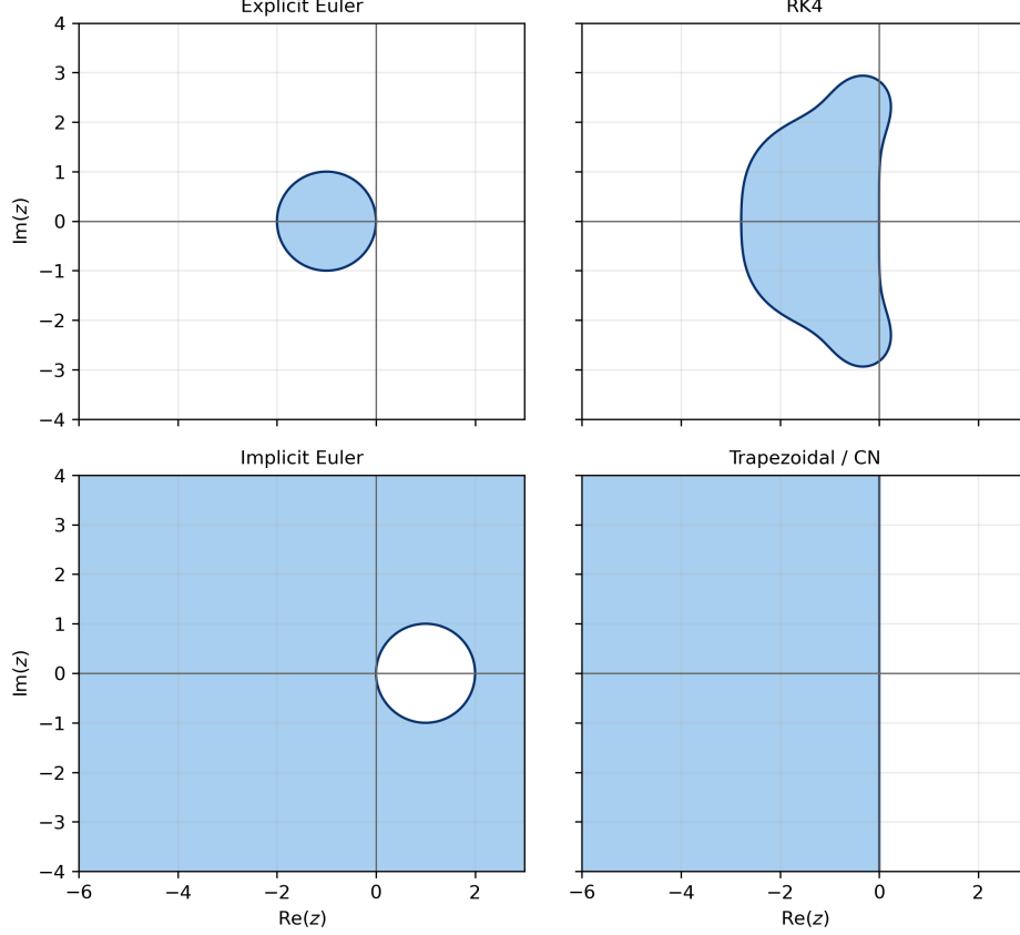
Figure 3: Absolute-stability regions |R(z)| \leq 1 (shaded) of the four integrators on the common domain \text{Re } z \in [-6, 3] , \text{Im } z \in [-4, 4] .
