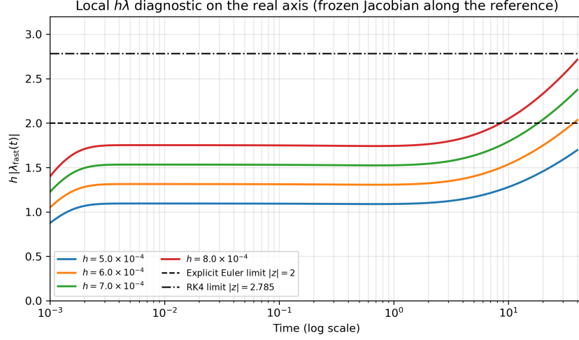
Figure 6: Local h\lambda diagnostic on the real axis: h|\lambda_{\text{fast}}(t)| along the reference trajectory for four step sizes, against the real-axis limits of Explicit Euler (2) and RK4 (2.7853). A curve above a limit means that the frozen-Jacobian condition is violated at that time.
