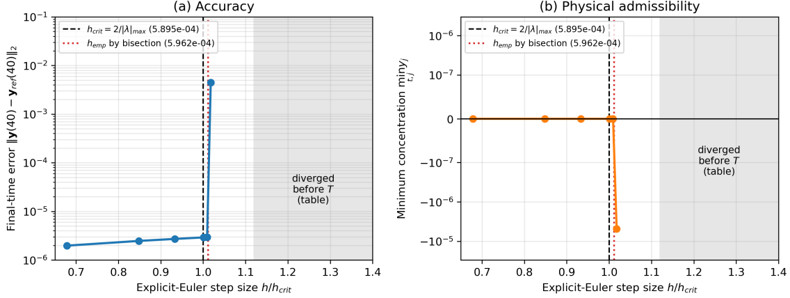
Figure 9: Explicit Euler near h_{crit} . (a) final-time error; (b) minimum concentration over the run. The step size is scaled by h_{crit} ; the shaded region contains the diverged runs h = 7 \times 10^{-4} , 8 \times 10^{-4} (Table 5).
