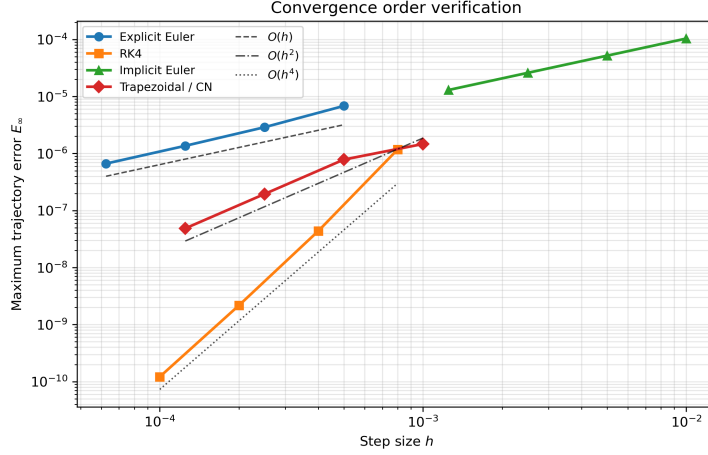
Figure 8: Convergence orders with respect to E_\infty . The dashed, dash-dotted and dotted lines are slope guides of order 1, 2 and 4.
