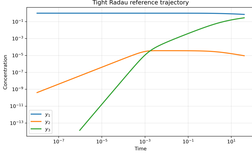
Figure 7: Tight Radau reference trajectory (values below \text{atol} = 10^{-14} are not drawn). y_2 stays several orders of magnitude below y_1 for all t , and below y_3 for t \gtrsim 2 \times 10^{-3} .
