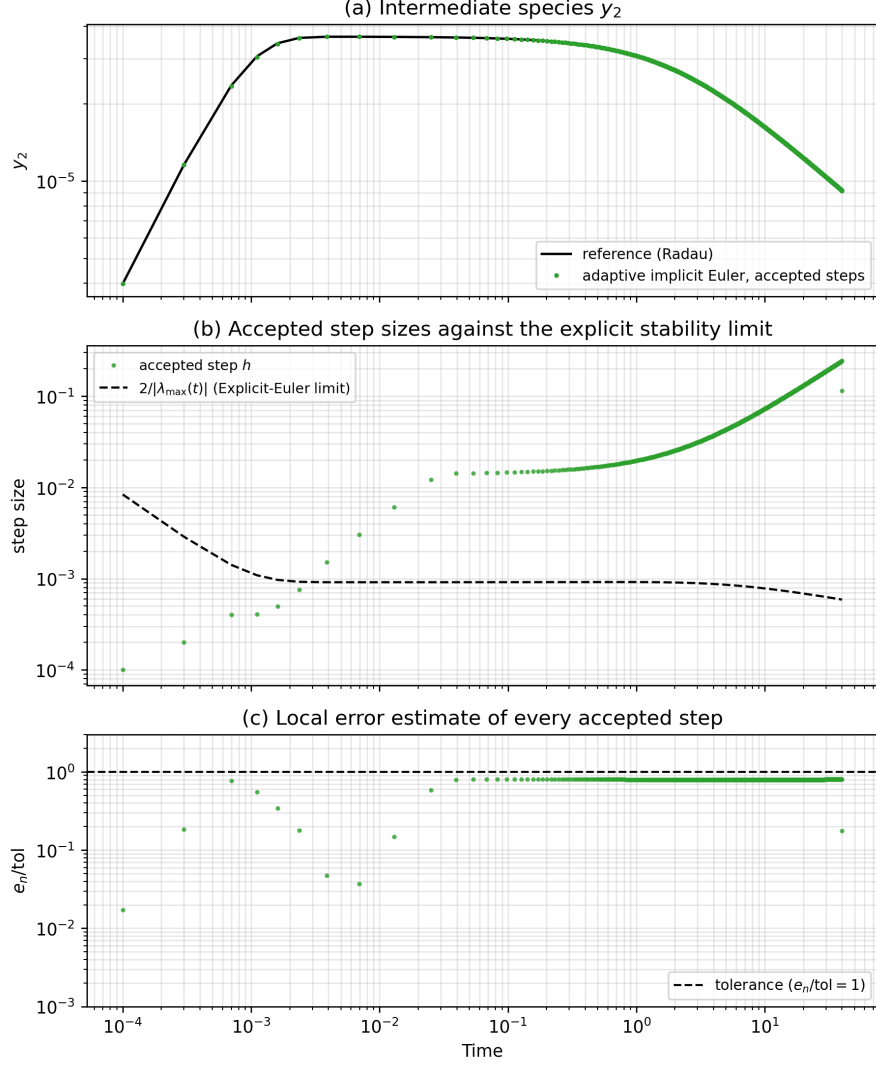
Figure 2: Self-implemented adaptive Implicit Euler with local extrapolation, \text{tol} = 10^{-6} . (a) Intermediate species against Radau. (b) Accepted macro-step sizes against the explicit stability bound. (c) The first-order step-doubling proxy in units of tolerance; it is not the local error of the extrapolated state.
