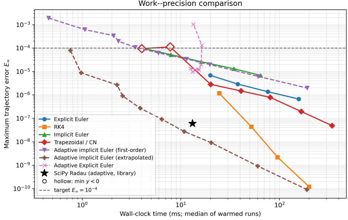
Figure 11: Work-precision diagram including the four fixed-step methods, adaptive EE, and both self-implemented adaptive IE variants. Hollow markers flag negative concentrations in the fixed-step runs. The star is SciPy Radau with \text{rtol} = 10^{-6} , \text{atol} = 10^{-9} , retained as a library baseline.
