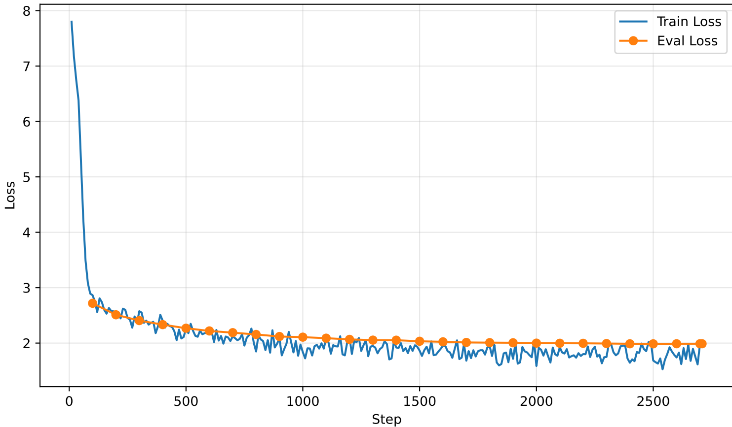
SFT Training and Evaluation Loss
