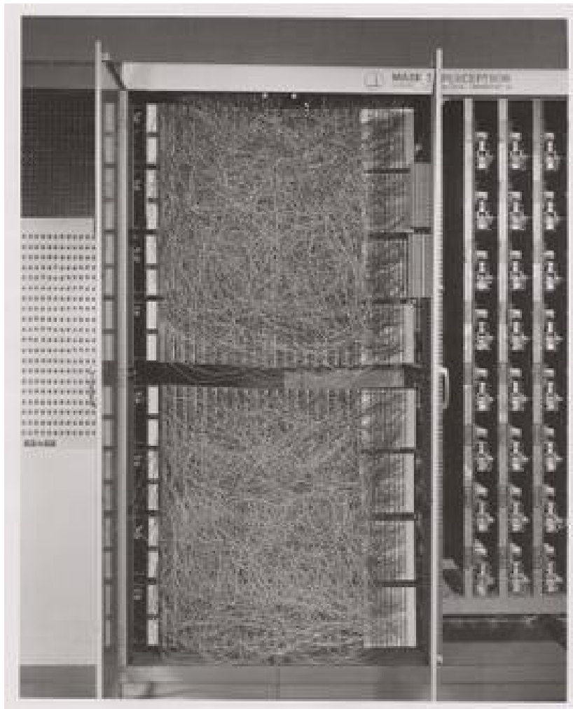
Figure 4.4: The Mark I computer for computing the perceptron's activity. Details can be found on Wikipedia's page.
