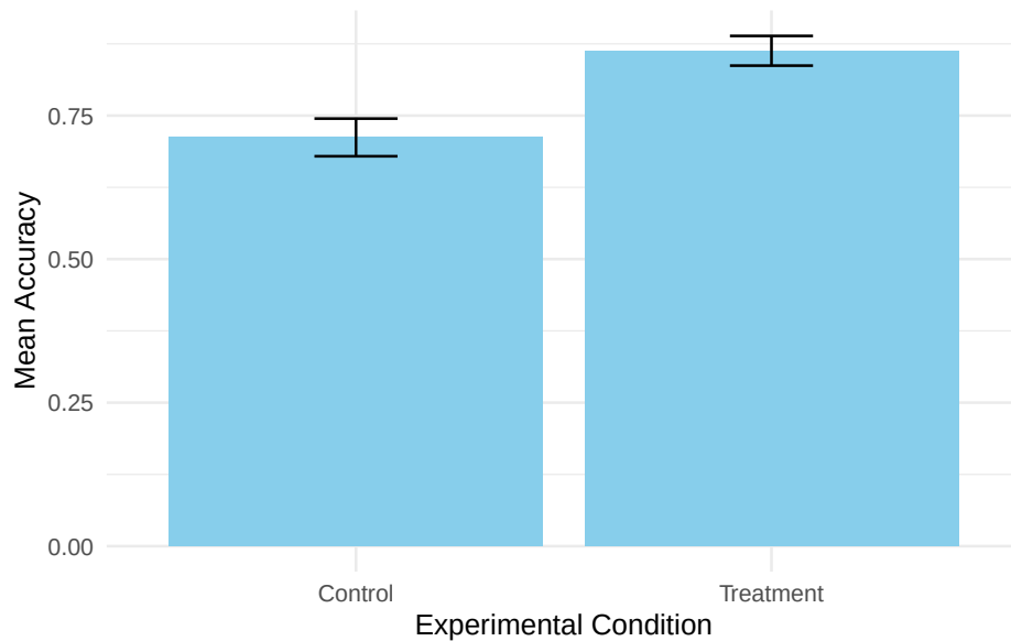
Figure 12.1: Mean Accuracy Scores by Condition (Treatment vs. Control)
