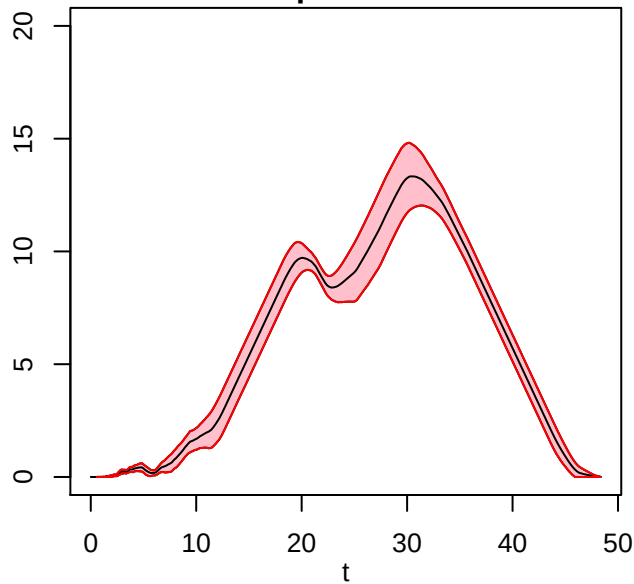
Mean 1st Landscape (n=30) with Adaptive 80% band
