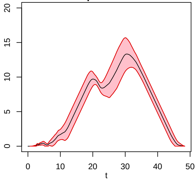
Mean 1st Landscape (n=30) with Adaptive 99.9% band
