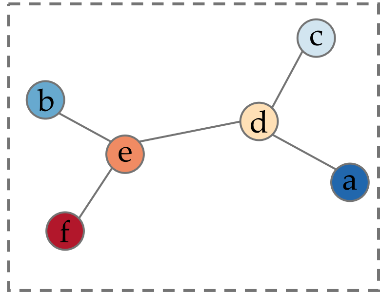
Graph
