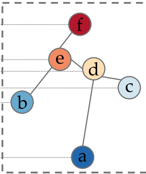
Merge Tree
