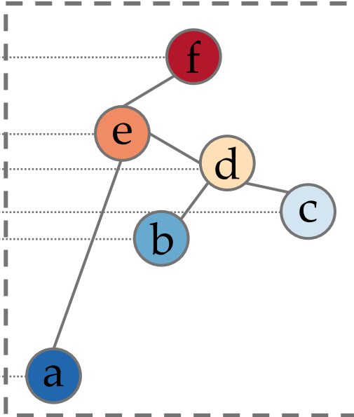
Merge Tree
