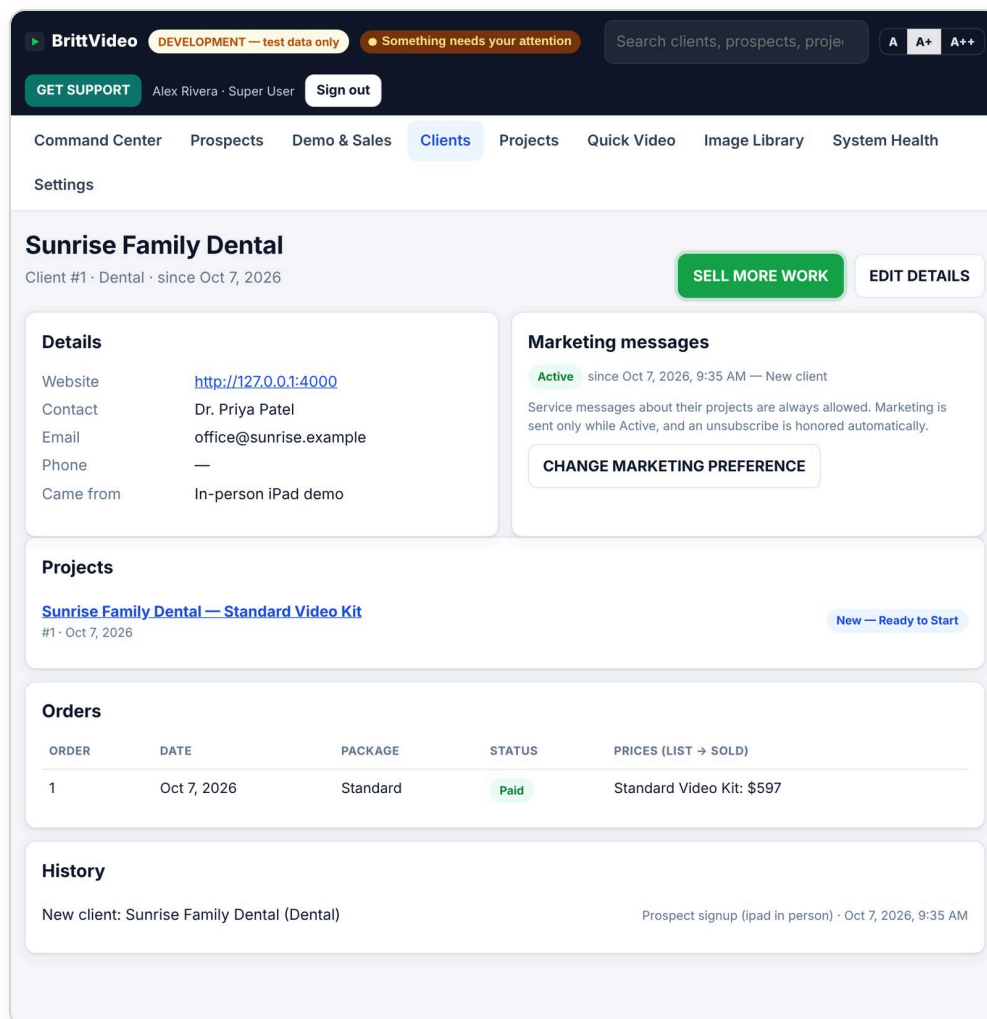
The client page.
