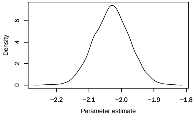
Density – lp[1, 1]
