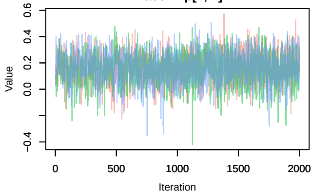
Trace – \text{lp}[3, 1]
