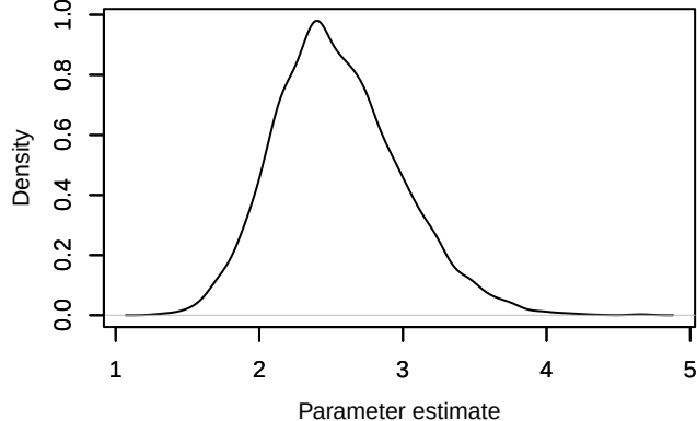
Density – \nu[1]
