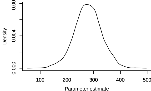
Density – dE[1]
