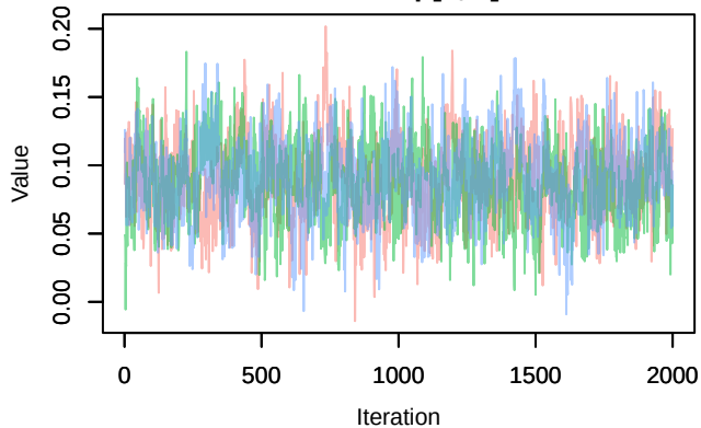
Trace – \text{lp}[1, 2]
