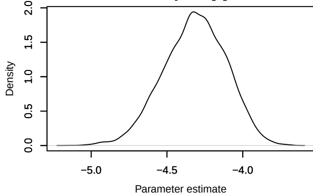
Density – a0[1]
