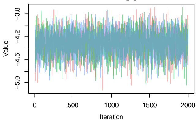
Trace – a0[1]
