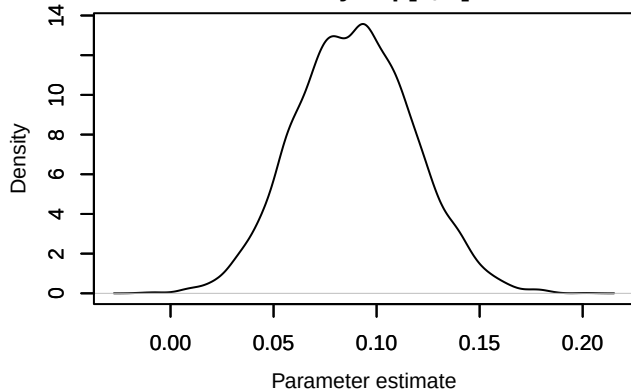
Density – \text{lp}[1, 2]
