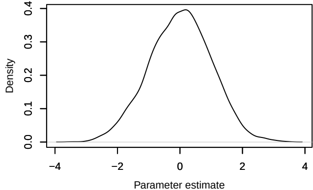
Density – a1[2]
