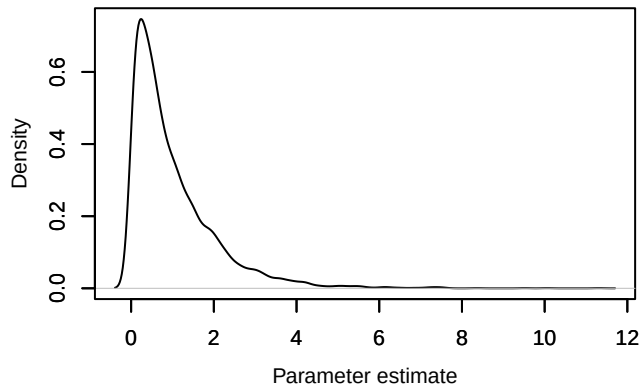
Density – U0[1, 1]
