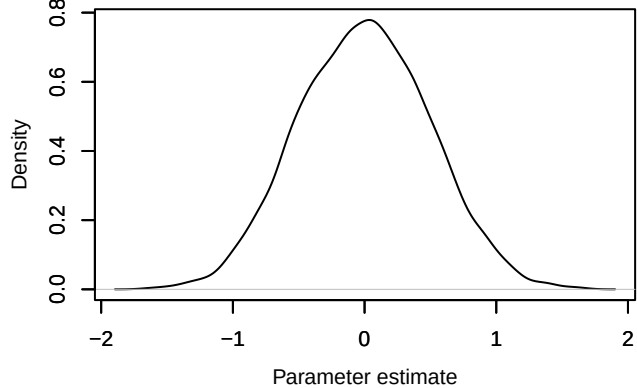
Density – eps_A_IP1_FY2022
