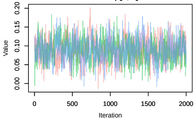
Trace – \text{lp}[1, 3]
