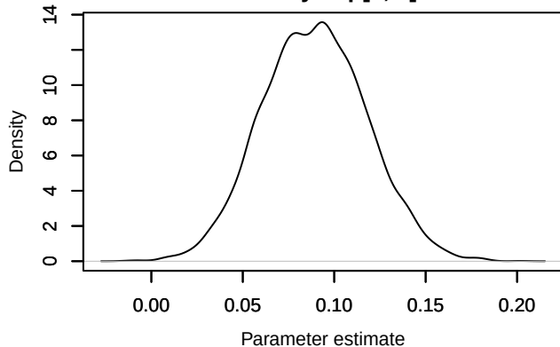
Density – \text{lp}[1, 3]
