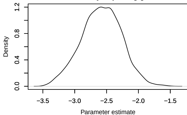
Density – IpsiLA[2]
