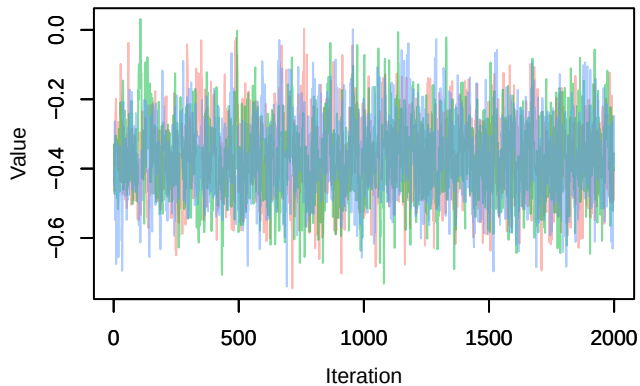
Trace – \text{lp}[3, 1]
