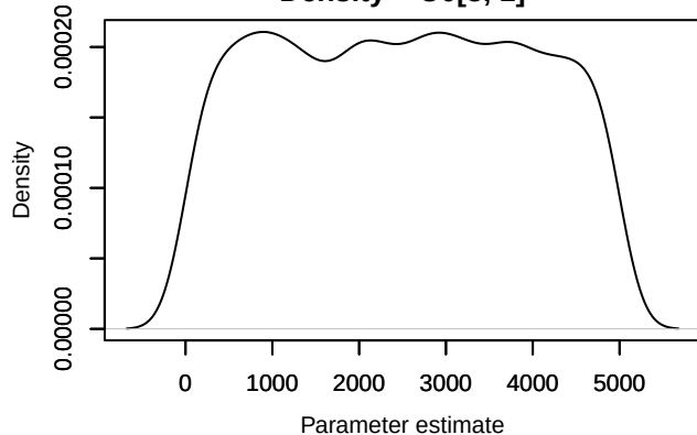
Density – U0[3, 1]
