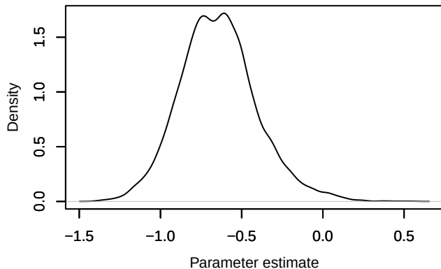
Density – lp[1, 1]
