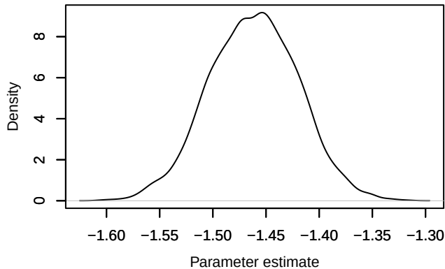
Density – lp[1, 1]
