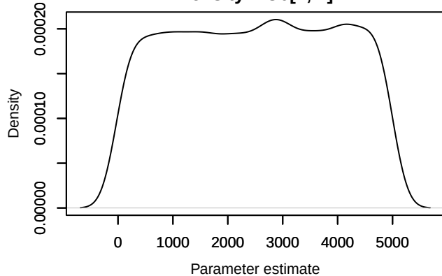
Density – U0[2, 1]
