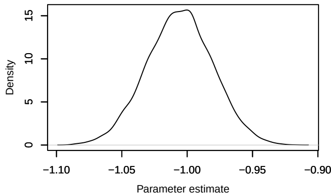
Density – \text{lp}[1, 2]
