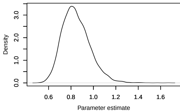
Density – dJ[1]
