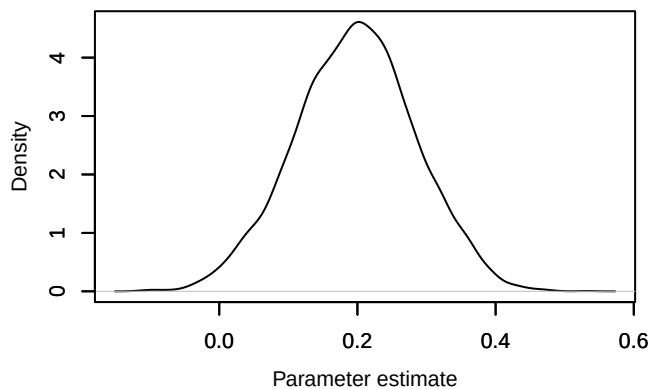
Density – dJ[1]
