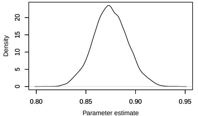
Density – g_eff[1]
