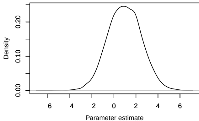
Density – lp_raw[1, 2]
