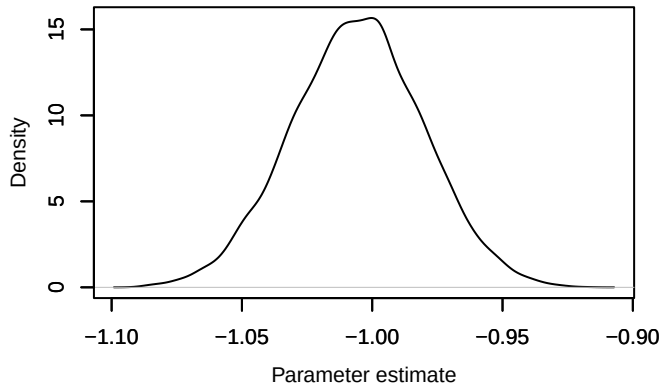
Density – lp_raw[1, 1]
