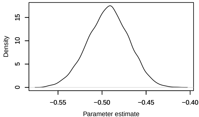
Density – lp_raw[3, 2]
