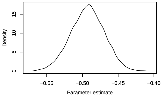
Density – lp[3, 2]
