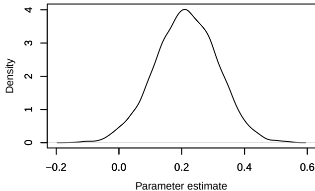
Density – \text{lp}[3, 1]
