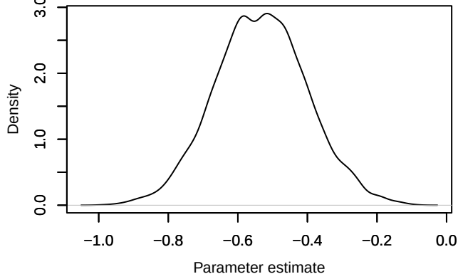
Density – lp[1, 1]
