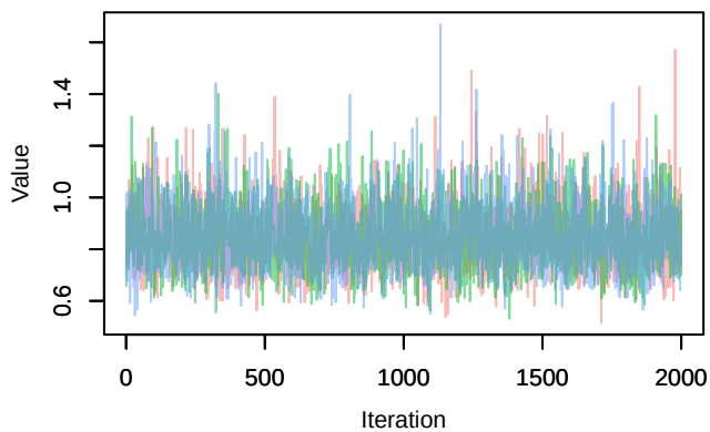
Trace – dJ[1]
