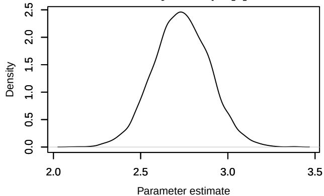
Density – sigma_phi[1]
