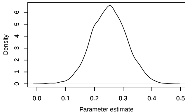
Density – lp_raw[1, 2]
