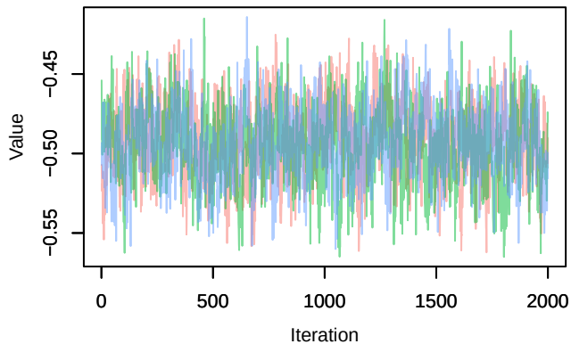
Trace – lp[3, 2]
