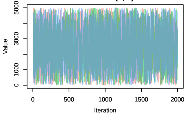
Trace – U0[3, 2]
