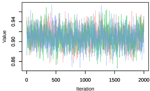
Trace – \text{g\_eff}[1]
