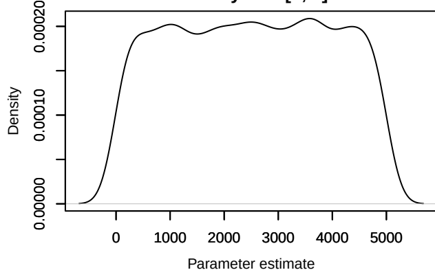
Density – U0[3, 2]
