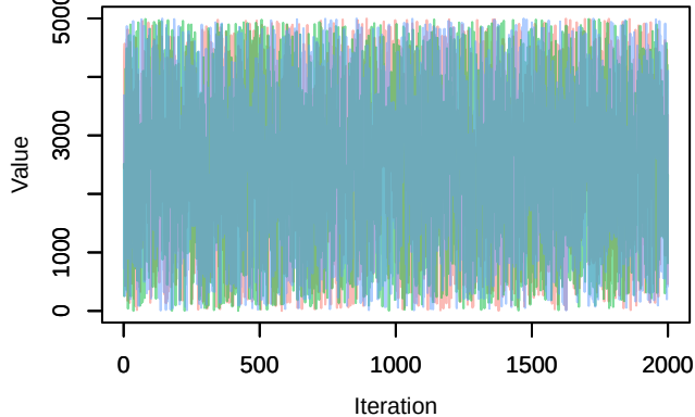
Trace – U0[3, 1]
