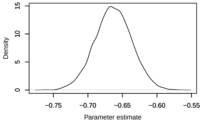
Density – \text{lp}[3, 2]
