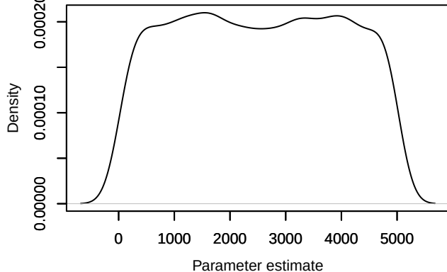
Density – U0[3, 1]
