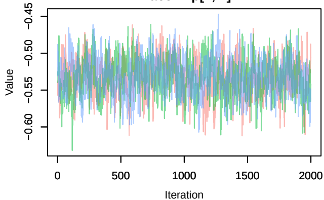
Trace – \text{lp}[3, 2]
