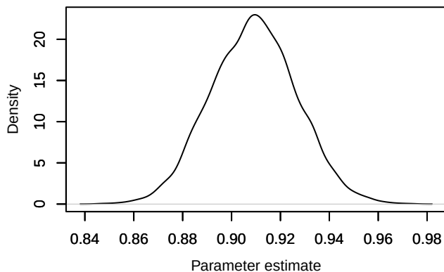
Density – \text{g\_eff}[1]
