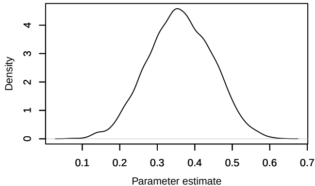
Density – dJ[1]
